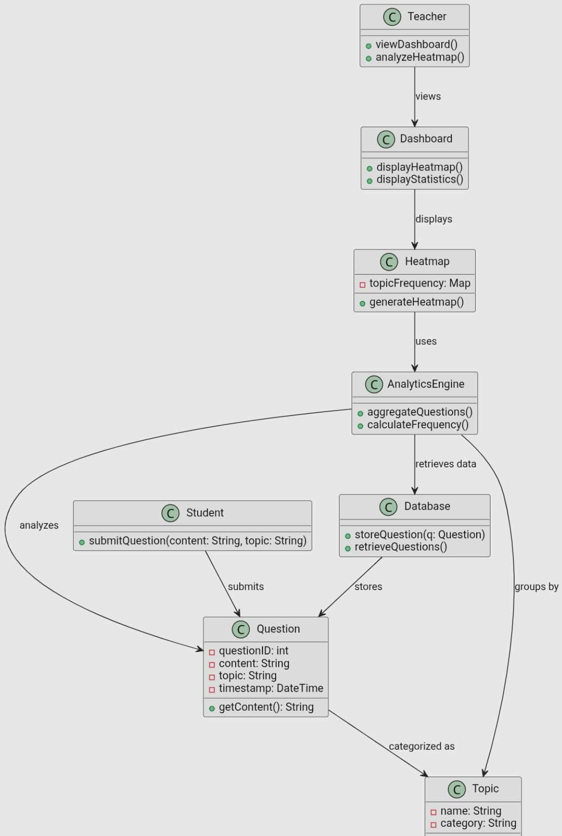
Incognito Intel - Class Diagram
