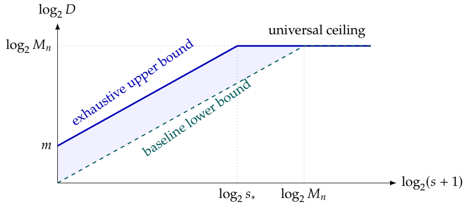
Figure 1: Schematic baseline bounds, suppressing additive constants on logarithmic axes. The shaded region represents a gap between bounds, not proved amplification. The lower bound is proved in Proposition 9.1. The structural bounds in Sections 4 and 5 can improve the upper curve.
