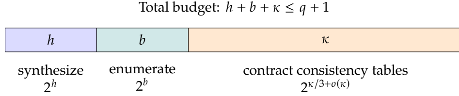
Figure 2: The limiting balance is h : b : \kappa = 1 : 1 : 3 . All three exponents then approach (q + 1)/5 . This balances upper bounds; it supplies neither a hard example nor a proof that this rate is optimal. Ordinary preprocessing costs p additional gates, once.
