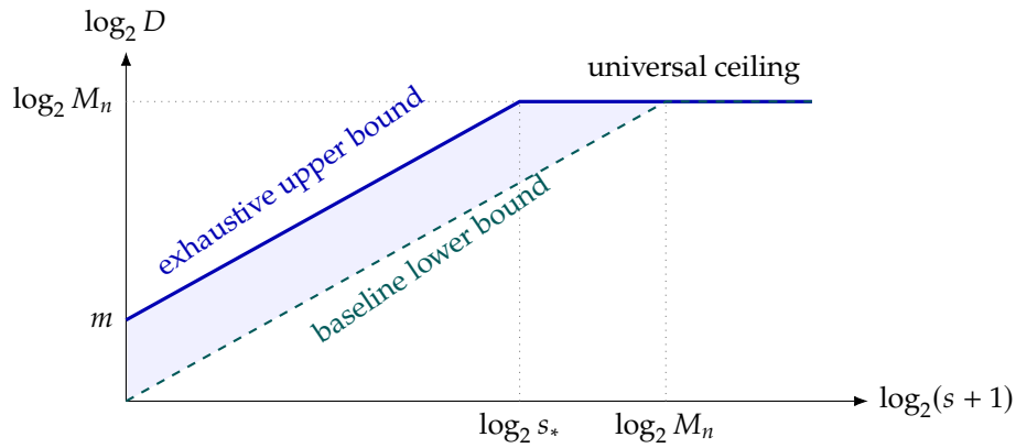
Figure 2: Schematic baseline bounds, suppressing additive constants on logarithmic axes. The shaded region represents a gap between bounds, not proved amplification. The lower bound is proved in Proposition 13.1. The structural bounds in Sections 6 and 7 can improve the upper curve.
