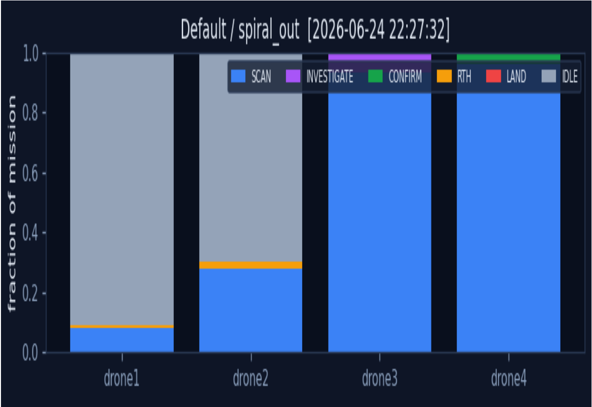
Per-drone task histogram
