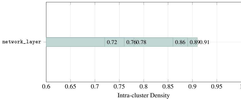
Figure 22: Cluster density at equilibrium (19 patterns, 6 clusters). The density gradient reflects semantic tightness: DNS pairs form the densest cluster, while network-layer patterns bridge clusters.
