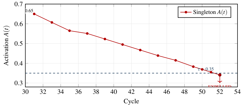
Figure 18: Singleton trajectory: activation decay from u_0 = 0.65 (cycle 31) to expulsion at A = 0.341 < \tau (cycle 52). Net suppression force: -0.014/\text{cycle} from four lateral inhibitors.
