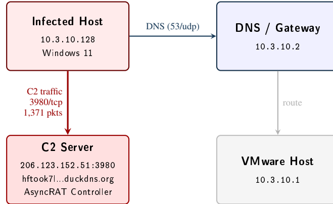
Figure 21: Network topology extracted by the pcap_analyzer field. Bold red arrow indicates the primary C2 channel (11.8% of all traffic, ~19 minutes continuous).
