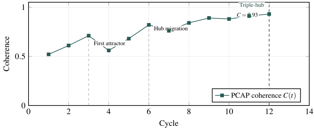
Figure 23: Coherence evolution for the pcap_analyzer session over 12 cycles. Dips at cycles 4 and 7 correspond to new-wave injection (coherence reset); recovery is rapid due to strong resonance with existing structure.
