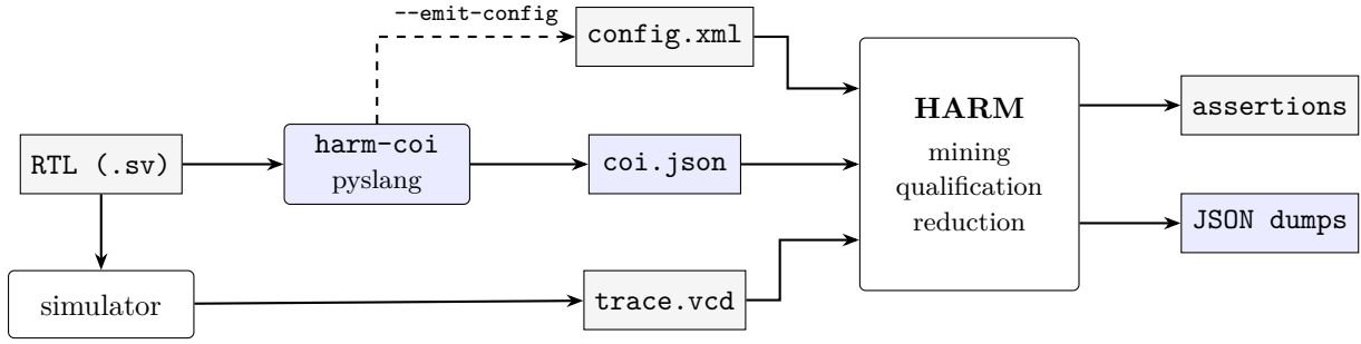
Figure 1: The tool flow of HARM v4. New parts are shaded. The RTL is optional: without it, HARM works as in v3 on traces and hints only.
