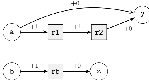
Figure 3: The multipath fixture. Edges carry their register delays; the cone of y contains a at depths 0 and 2, r1 at depth 1 and r2 at depth 0. b cannot influence y .
