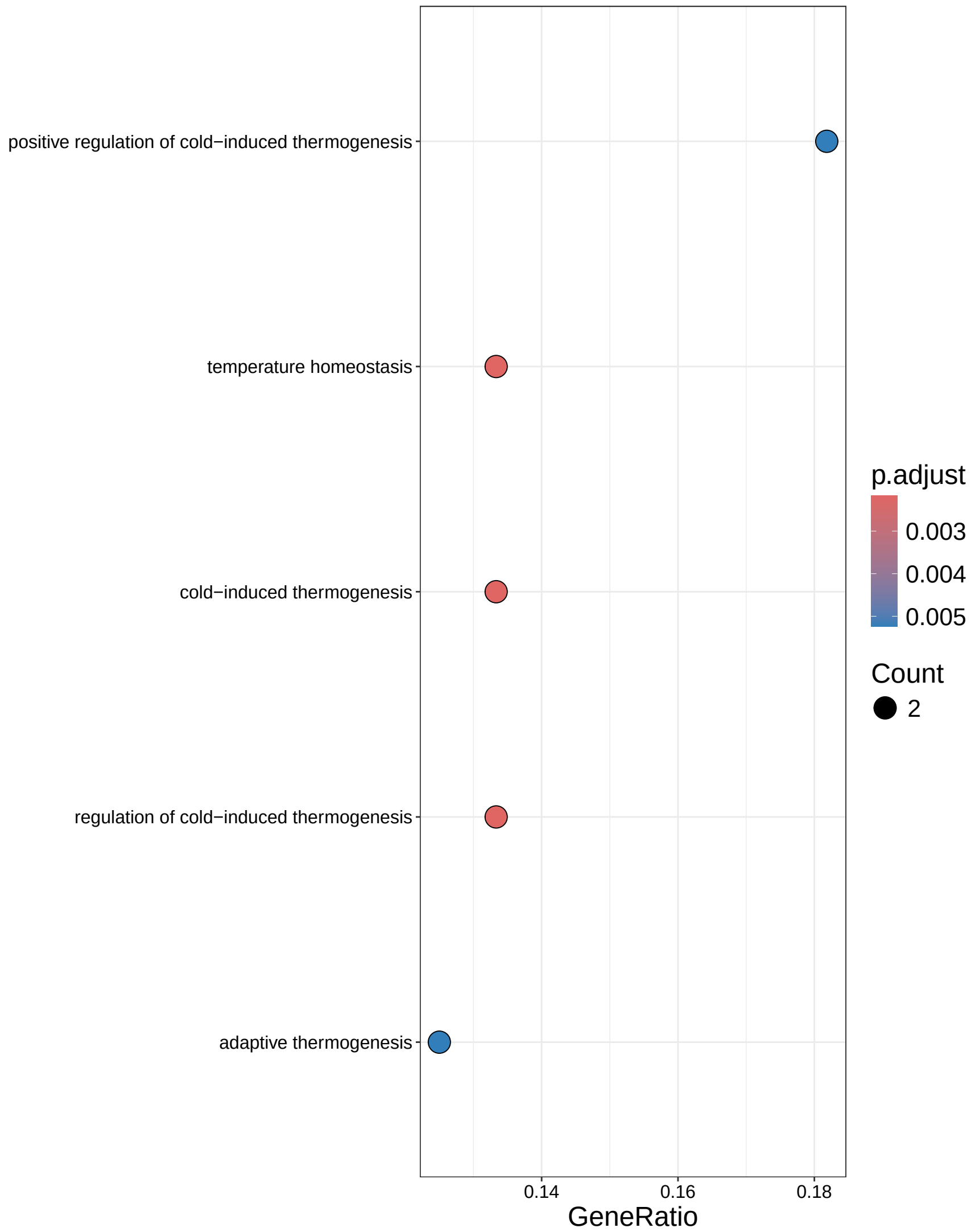
Biological processes enriched in Round Spermatids
