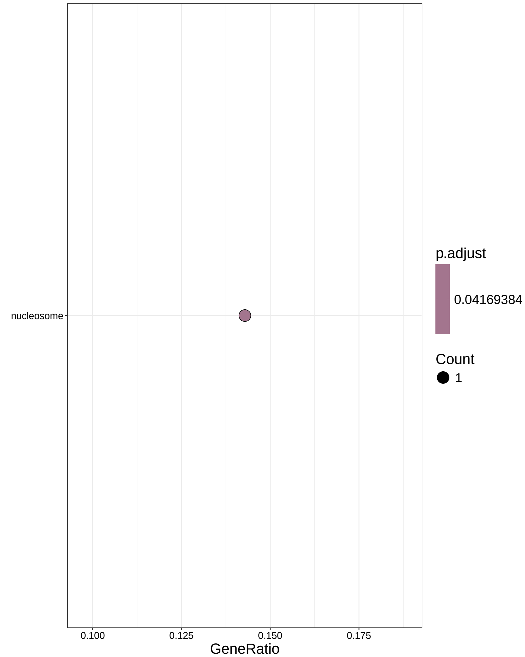
Cellular components enriched in Round Spermatids
