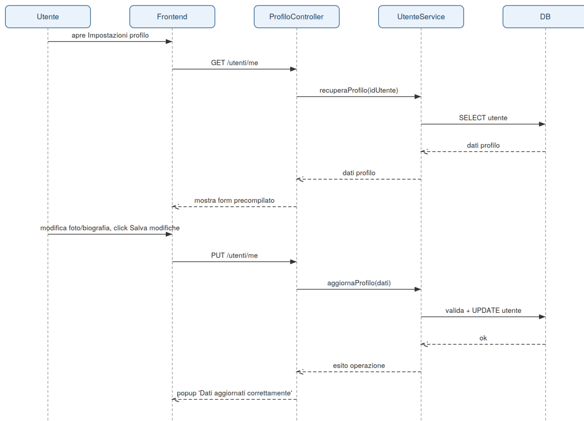
Sequence Diagram – UC_4 Modifica Dati Profilo
