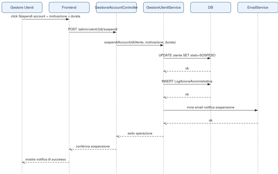
Sequence Diagram – UC_23 Sospensione Account
