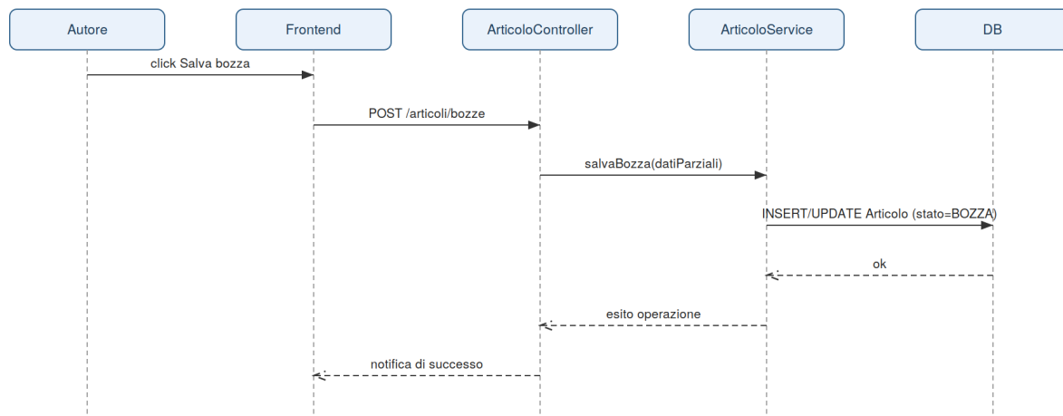
Sequence Diagram – UC_16 Salvataggio Bozza
