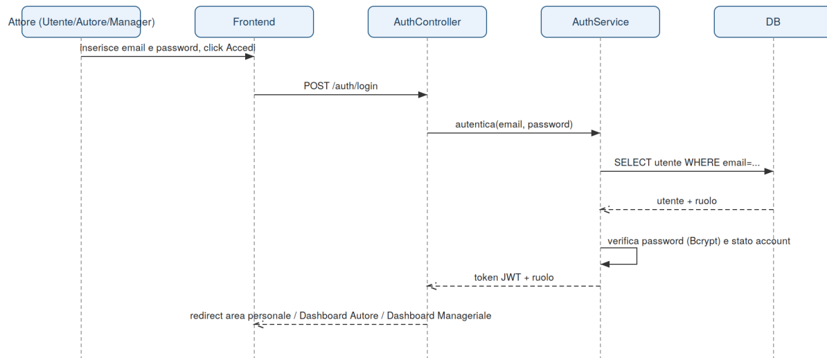
Sequence Diagram – UC_2 Login
