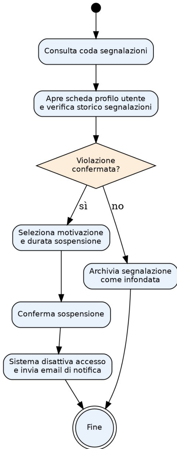
Activity Diagram - Sospensione
