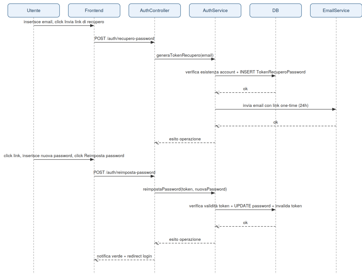
Sequence Diagram – UC_3 Recupero Password
