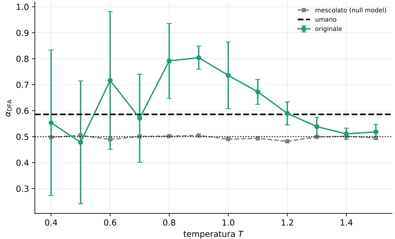
Esponente DFA — Qwen2.5-1.5B (cfr. [L] Fig. 4B)
