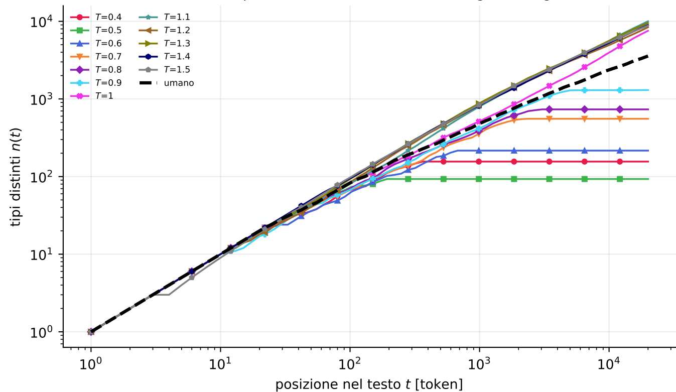
Curve di Heaps — Qwen3.5-4B-Base (cfr. [Z] Fig. 3, [L] Fig. 3A)
