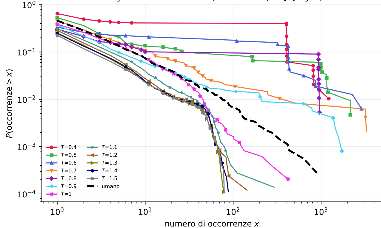
Istogramma cumulativo — Qwen2.5-3B (cfr. [Z] Fig. 6)
