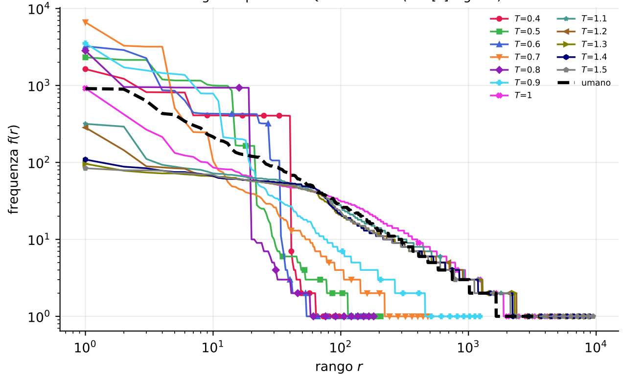
Rango-frequenza — Qwen2.5-3B (cfr. [L] Fig. 2A)
