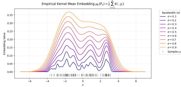
Figure 1: An Empirical Kernel Mean Embedding mapping discrete particles into a Reproducing Kernel Hilbert Space (RKHS). The bandwidth ( \sigma ) visually dictates the strictness of the RKHS smoothness penalty, illustrating how isolated data points are mathematically transformed into the continuous, interacting field that drives SVGD’s repulsive force.
