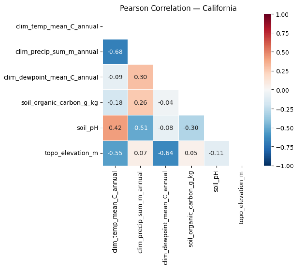
Figure 41: Pearson correlation heatmap: California.
