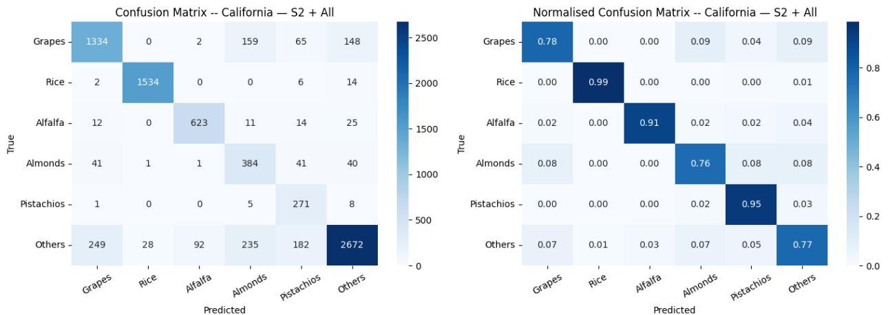
Figure 21: Part 2 confusion matrix for California: S2 + All covariates.
