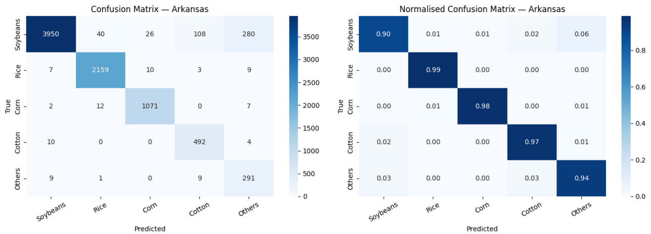
Figure 8: Part 1: Confusion matrix for Arkansas. The model achieves OA = 0.937 , with most errors concentrated in the Soybeans/Others boundary.
