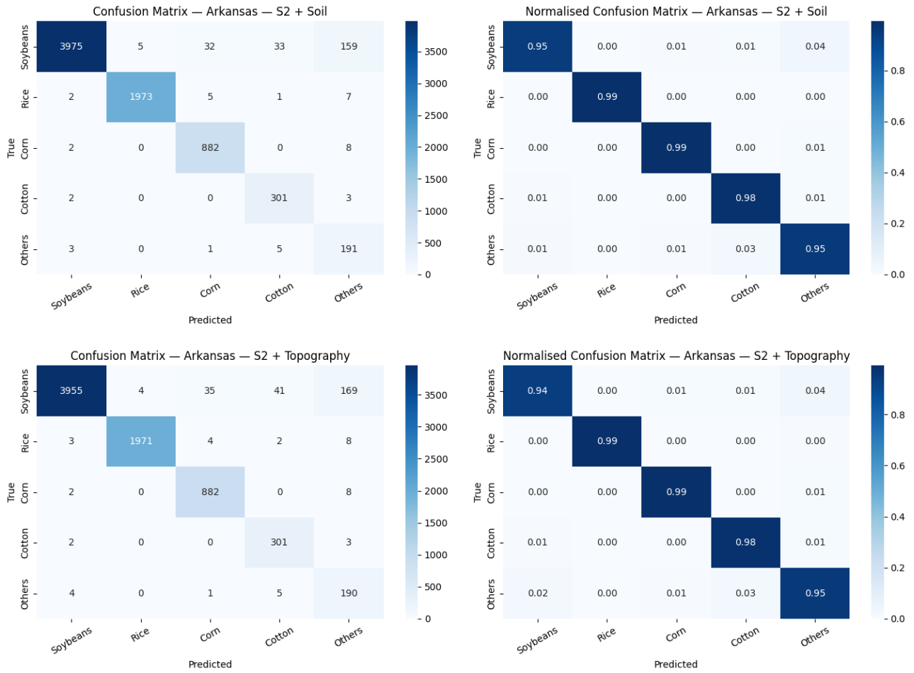
Figure 29: Part 3 confusion matrices for Arkansas: S2 + Soil (top) and S2 + Topo (bottom).
