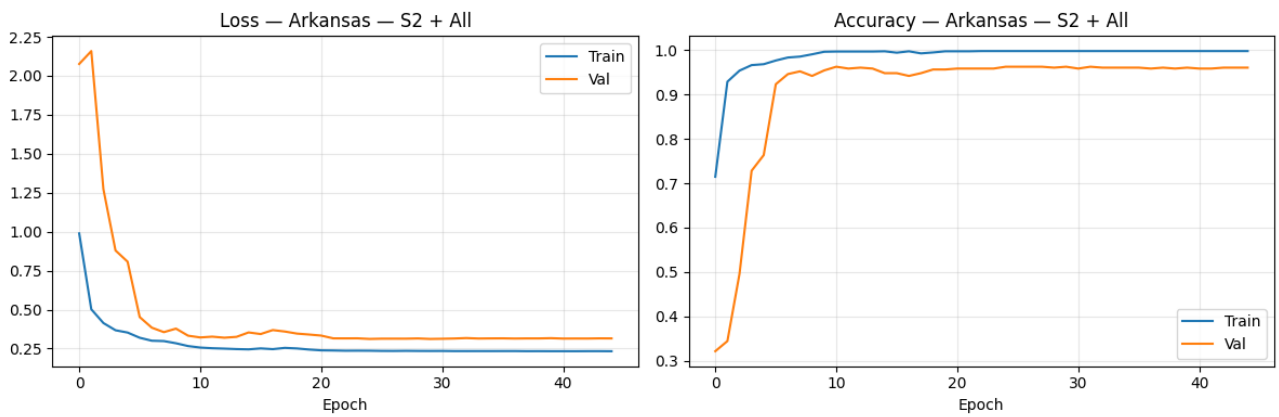
Figure 24: Part 3 convergence curves for Arkansas: S2 + All covariates.
