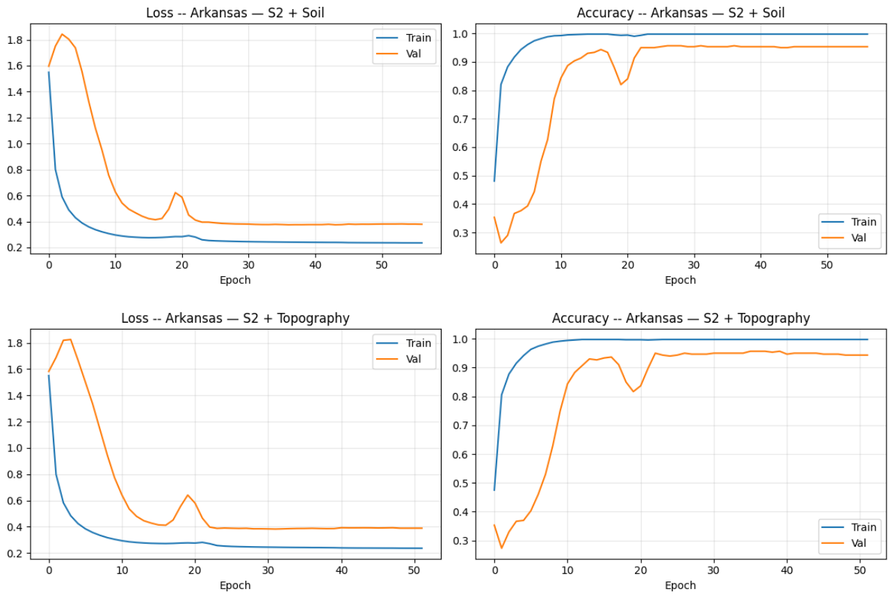
Figure 11: Part 2 convergence curves for Arkansas: S2 + Soil (top) and S2 + Topo (bottom).
