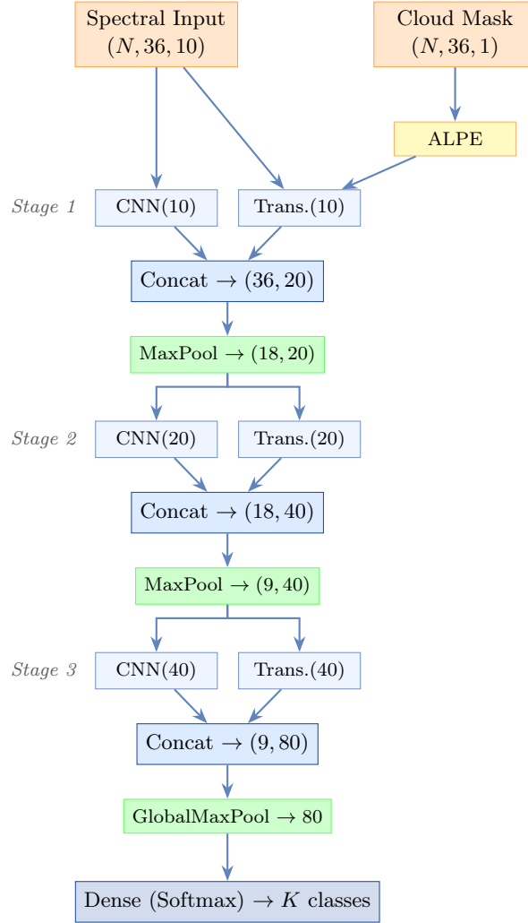
Figure 3: Baseline MCTNet architecture.
