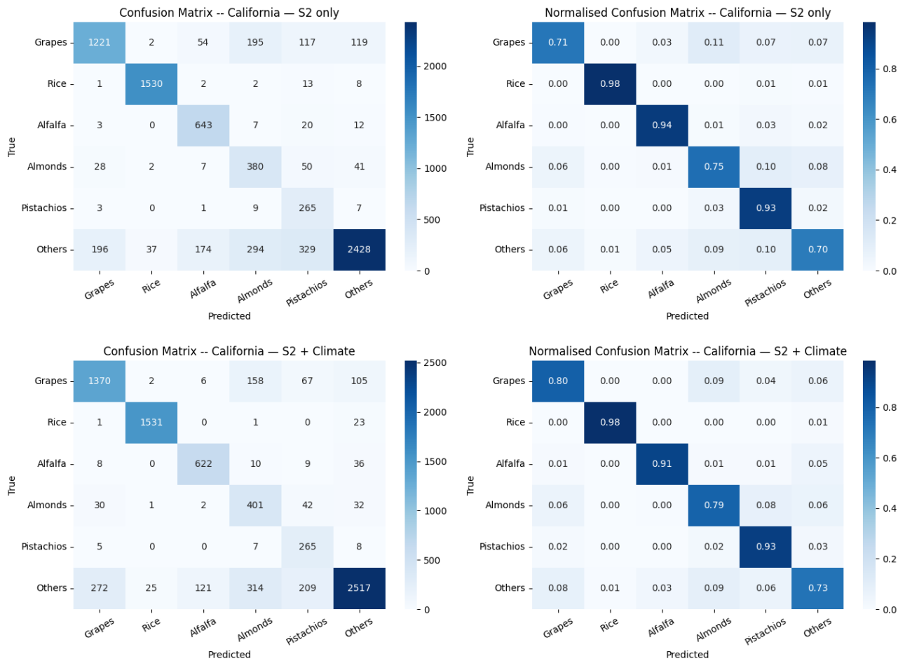
Figure 19: Part 2 confusion matrices for California: S2 Only (top) and S2 + Climate (bottom).
