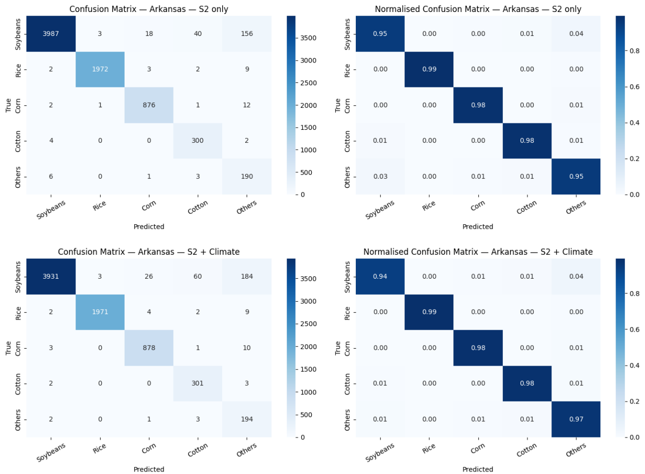
Figure 28: Part 3 confusion matrices for Arkansas: S2 Only (top) and S2 + Climate (bottom).
