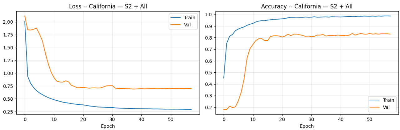
Figure 15: Part 2 convergence curves for California: S2 + All covariates.
