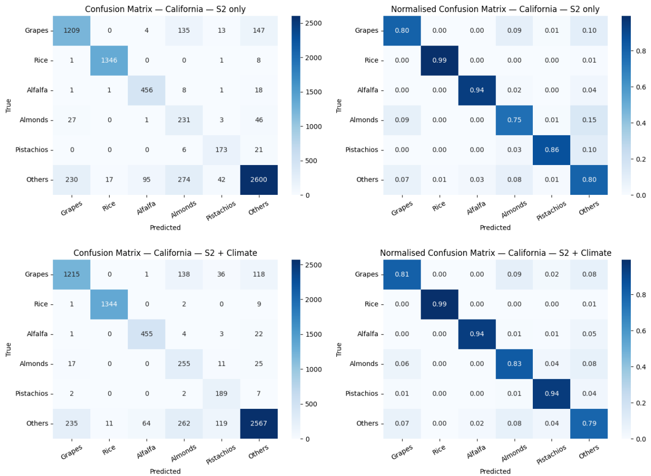
Figure 31: Part 3 confusion matrices for California: S2 Only (top) and S2 + Climate (bottom).
