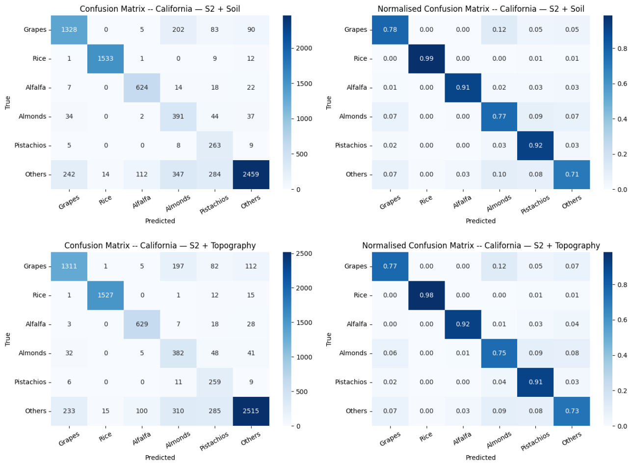
Figure 20: Part 2 confusion matrices for California: S2 + Soil (top) and S2 + Topo (bottom).
