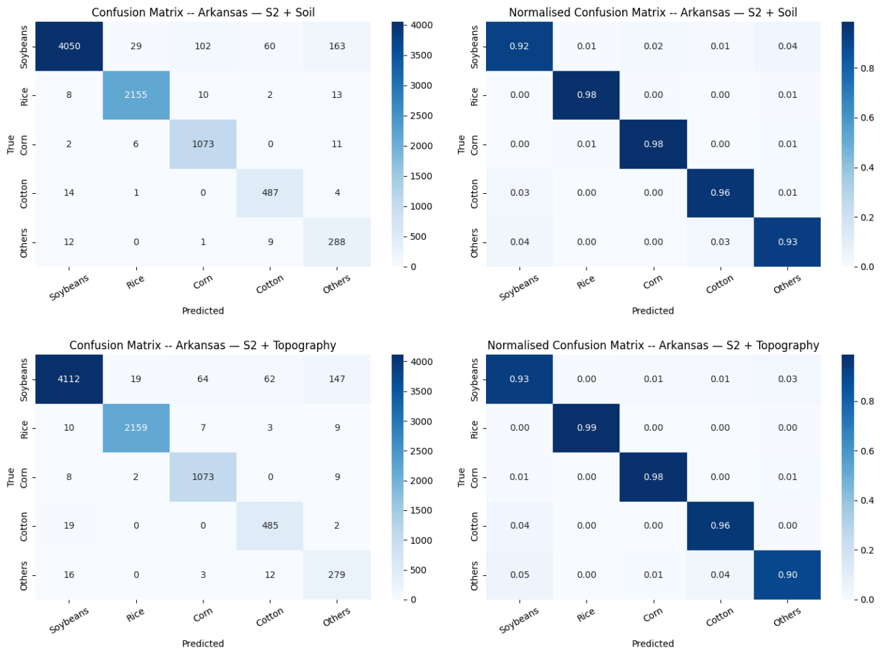
Figure 17: Part 2 confusion matrices for Arkansas: S2 + Soil (top) and S2 + Topo (bottom).
