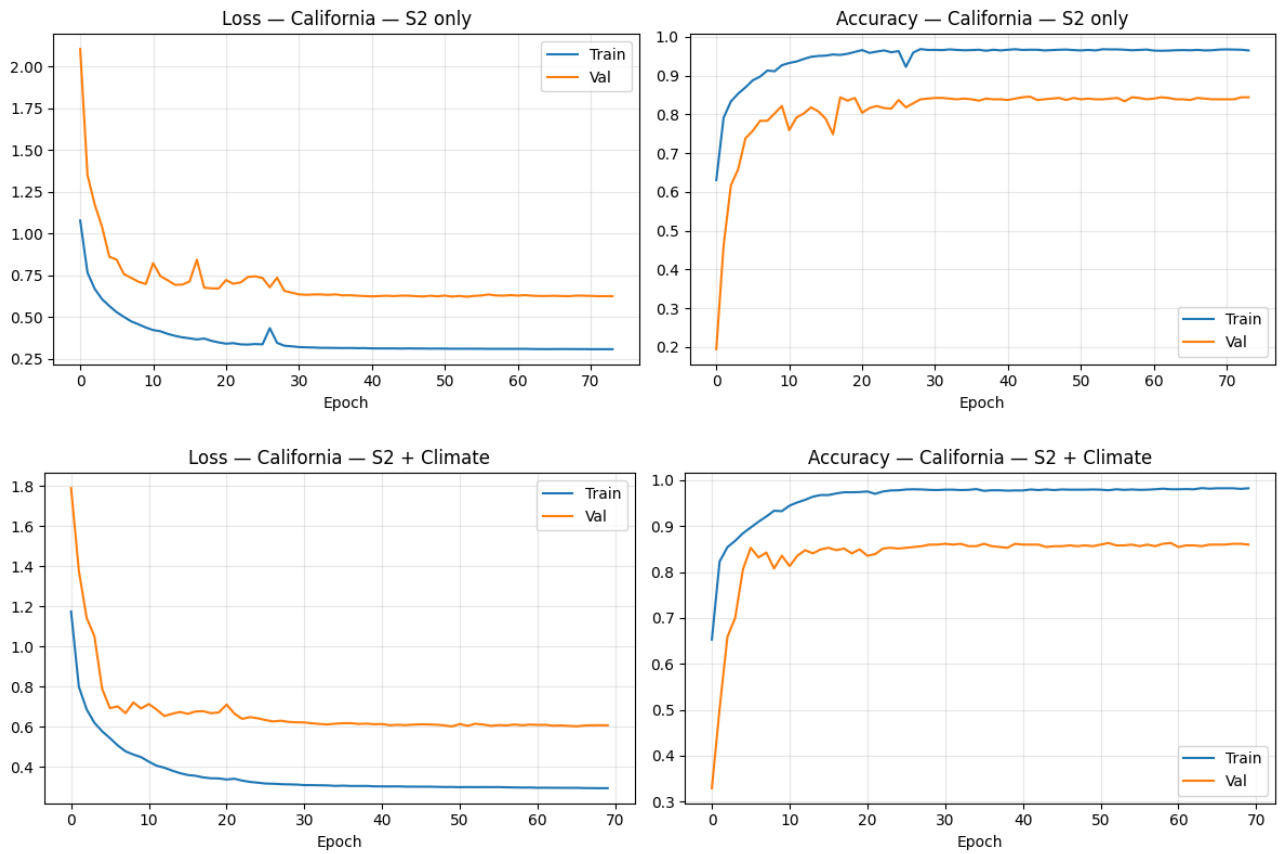
Figure 25: Part 3 convergence curves for California: S2 Only (top) and S2 + Climate (bottom).
