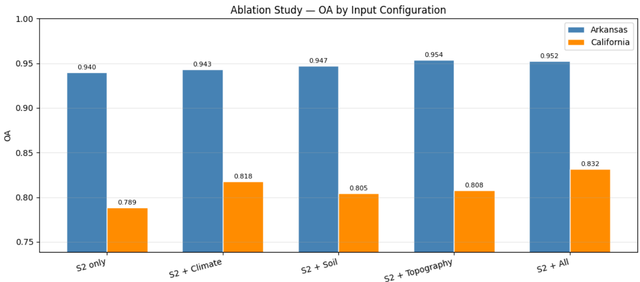
Figure 4: Part 2 ablation study: Overall Accuracy by input configuration for Arkansas and California. Training convergence curves and confusion matrices for each ablation configuration are provided in Appendix D.2.
