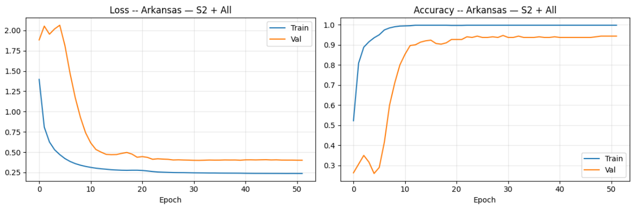
Figure 12: Part 2 convergence curves for Arkansas: S2 + All covariates.
