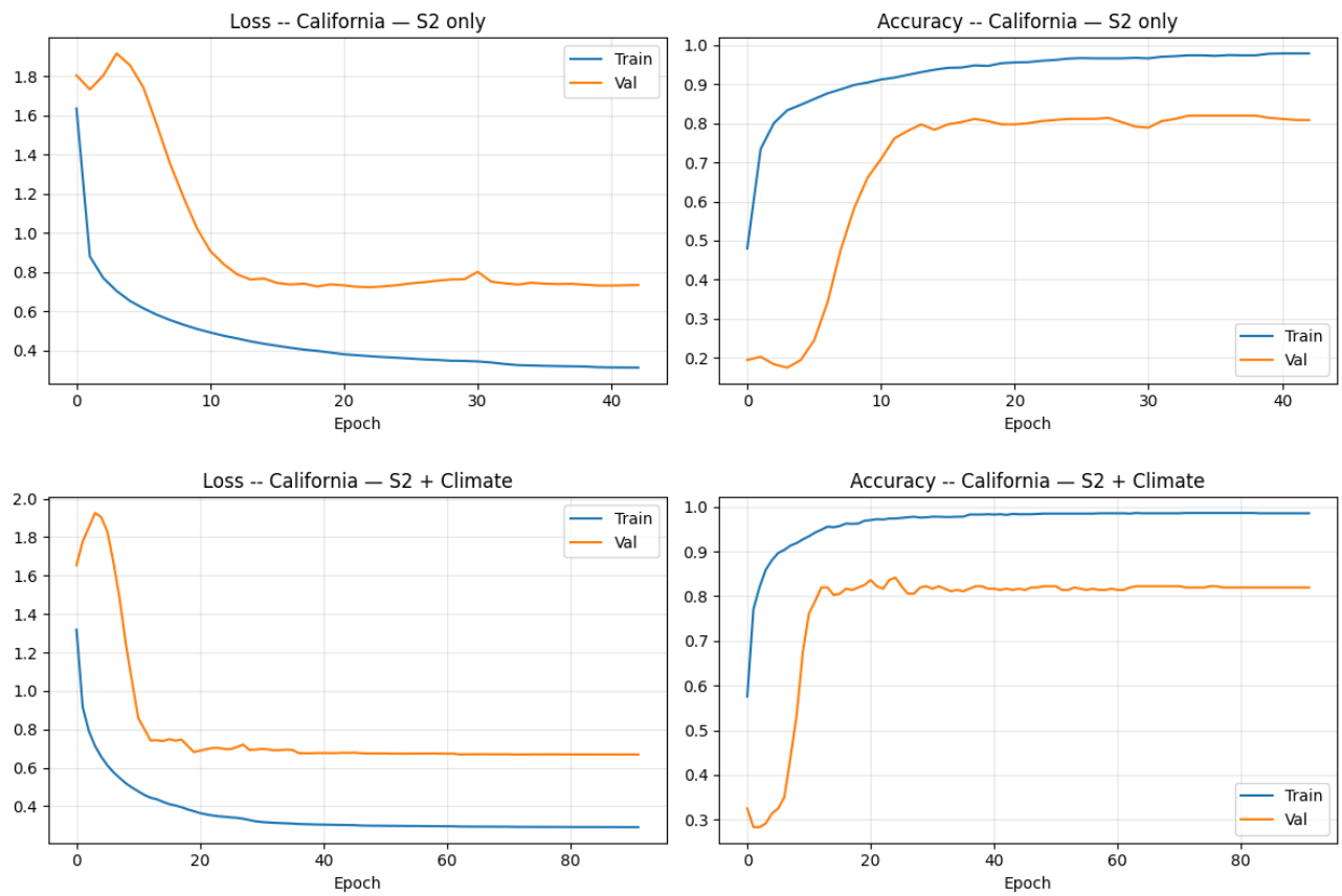
Figure 13: Part 2 convergence curves for California: S2 Only (top) and S2 + Climate (bottom).
