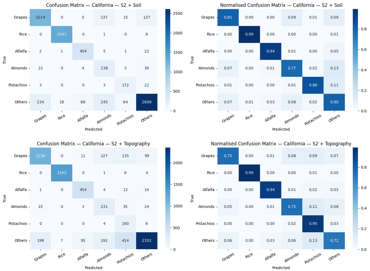
Figure 32: Part 3 confusion matrices for California: S2 + Soil (top) and S2 + Topo (bottom).
