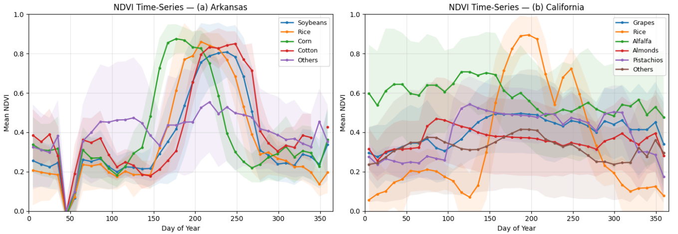
Figure 2: NDVI distribution in Arkansas and California.
