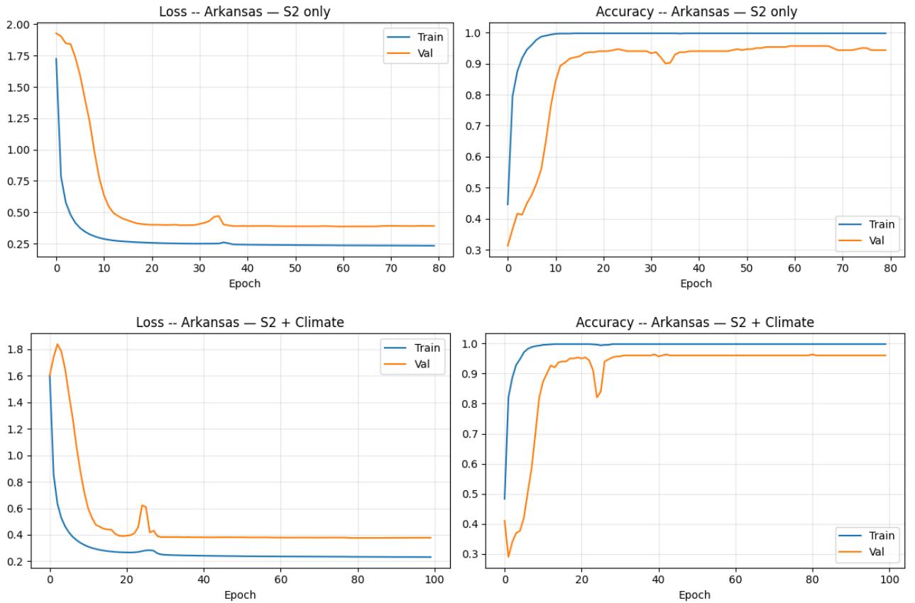
Figure 10: Part 2 convergence curves for Arkansas: S2 Only (top) and S2 + Climate (bottom).
