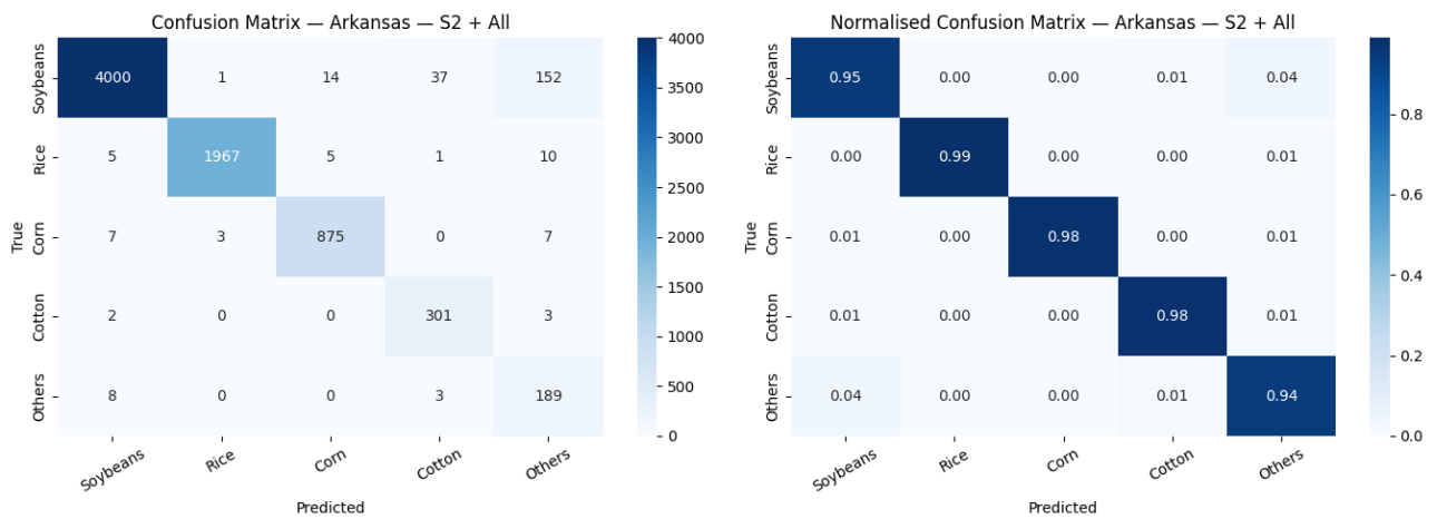
Figure 30: Part 3 confusion matrix for Arkansas: S2 + All covariates.
