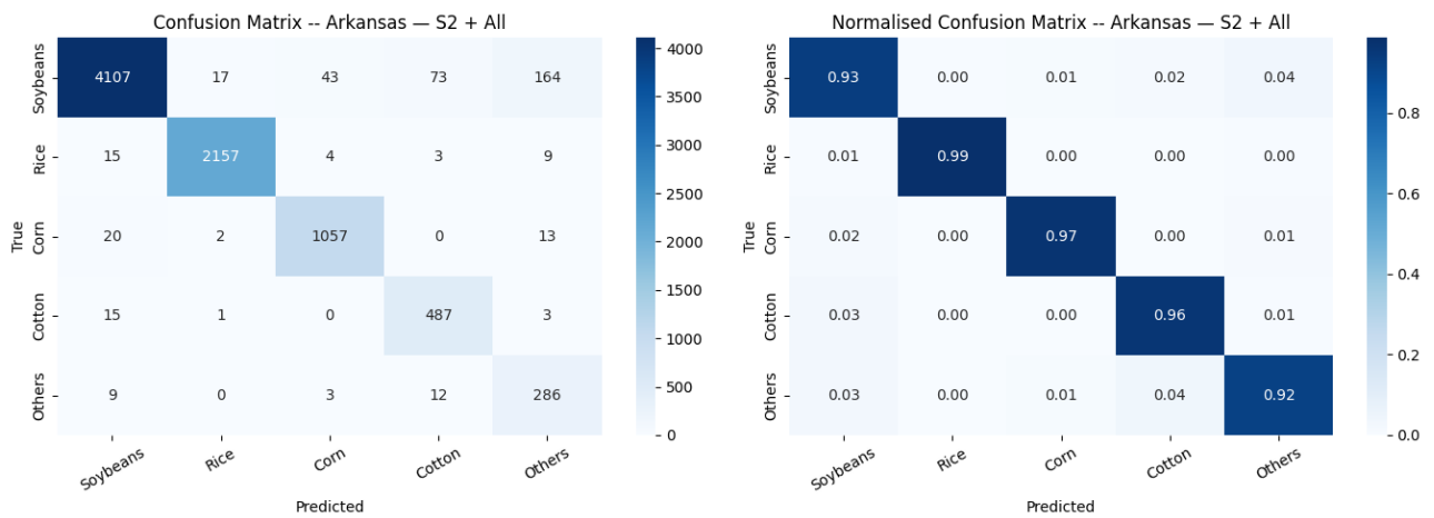
Figure 18: Part 2 confusion matrix for Arkansas: S2 + All covariates.
