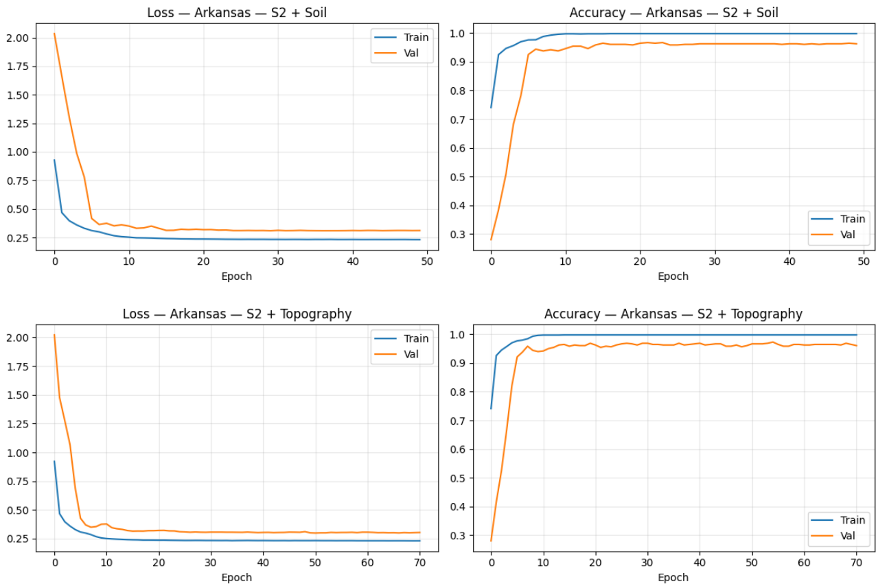
Figure 23: Part 3 convergence curves for Arkansas: S2 + Soil (top) and S2 + Topo (bottom).
