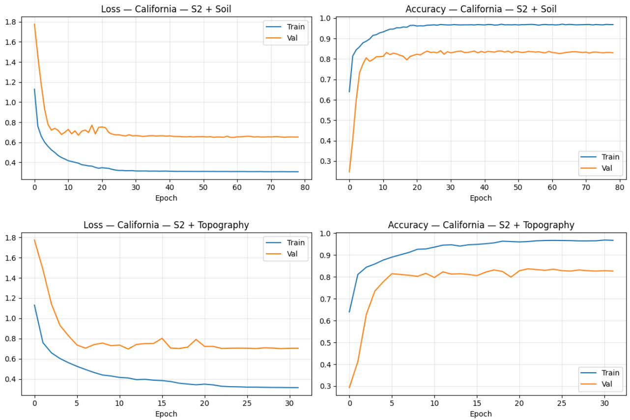
Figure 26: Part 3 convergence curves for California: S2 + Soil (top) and S2 + Topo (bottom).
