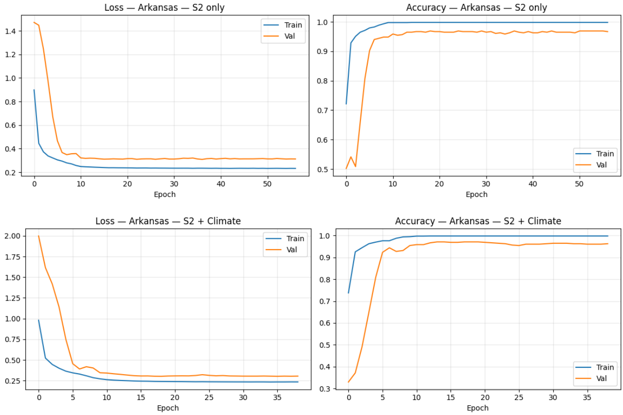
Figure 22: Part 3 convergence curves for Arkansas: S2 Only (top) and S2 + Climate (bottom).
