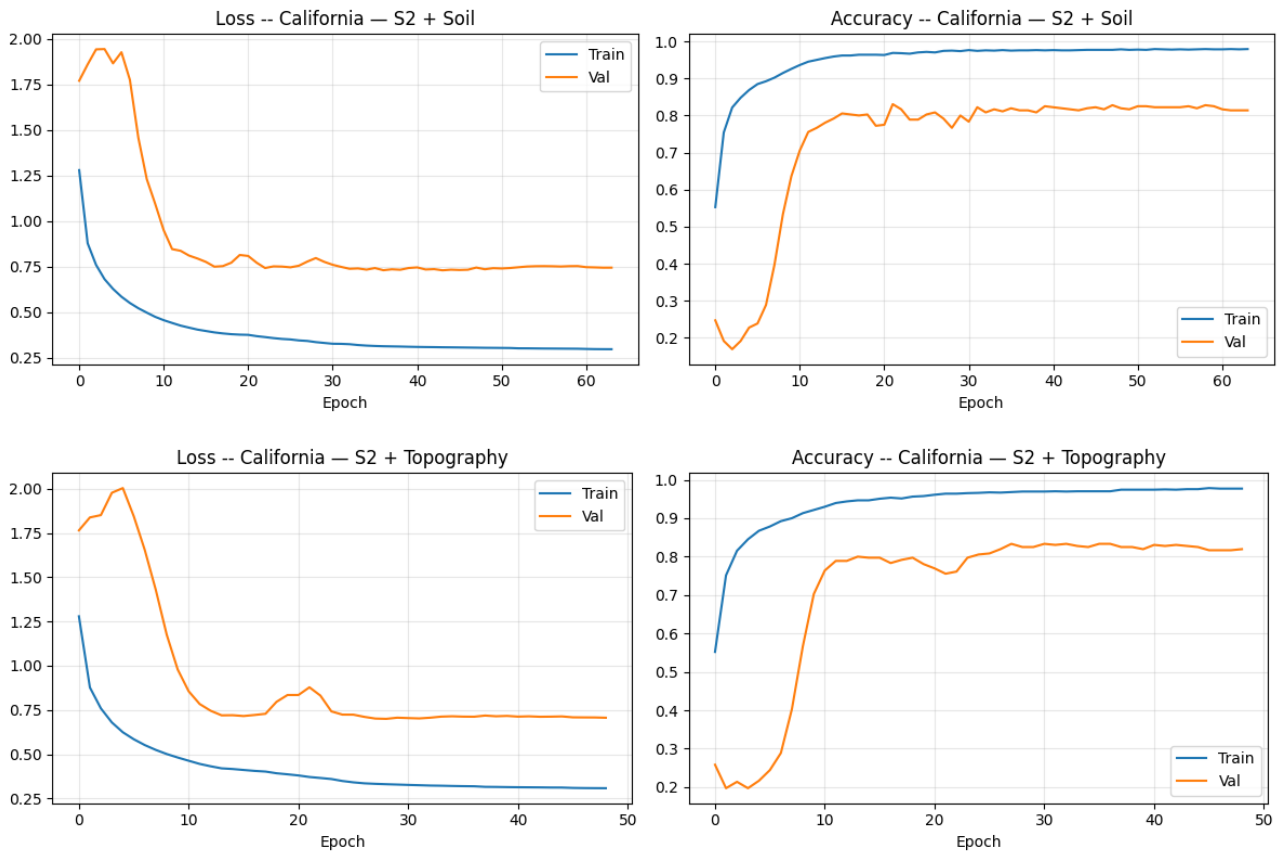
Figure 14: Part 2 convergence curves for California: S2 + Soil (top) and S2 + Topo (bottom).
