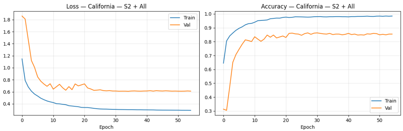
Figure 27: Part 3 convergence curves for California: S2 + All covariates.
