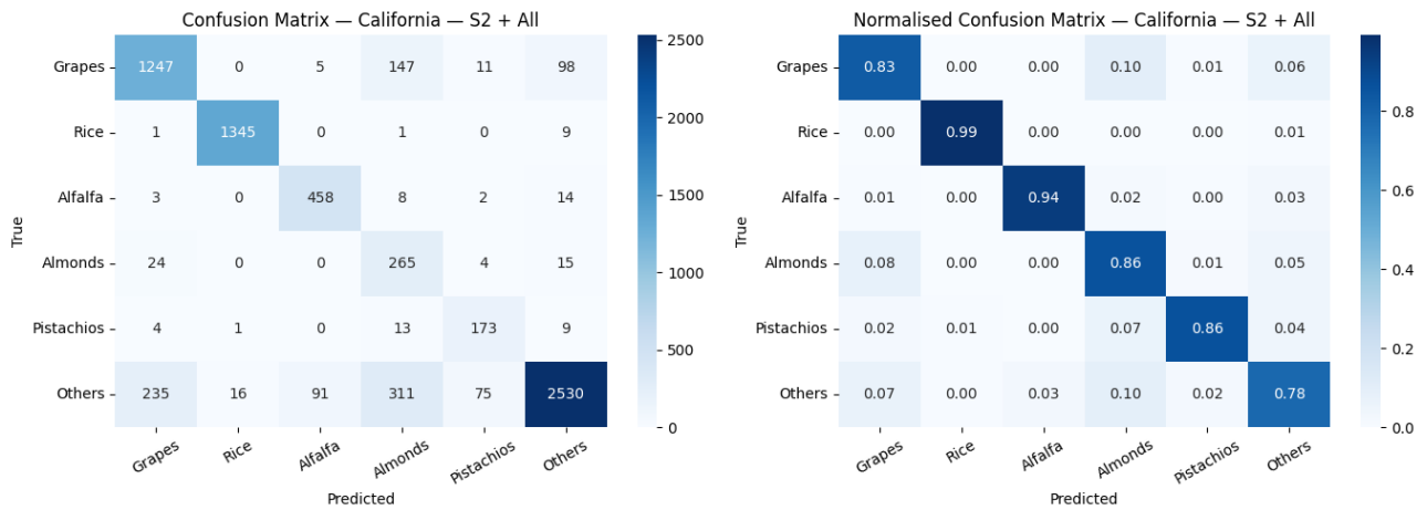
Figure 33: Part 3 confusion matrix for California: S2 + All covariates.
