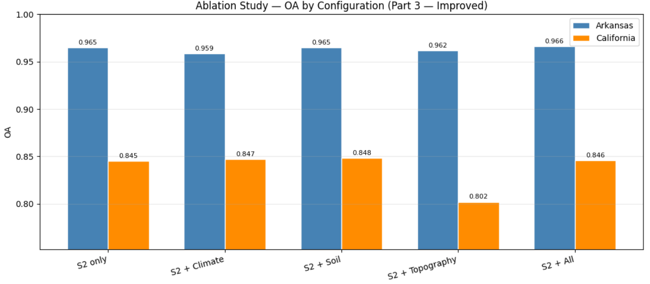
Figure 6: Part 3 ablation study: Overall Accuracy by input configuration for Arkansas and California. Training convergence curves and confusion matrices for each ablation configuration are provided in Appendix D.3.
