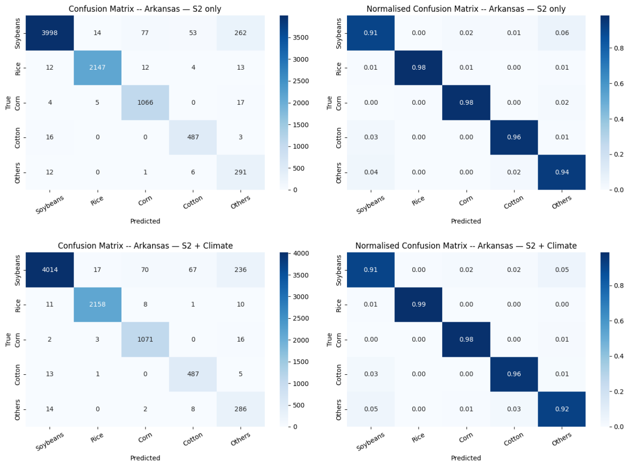
Figure 16: Part 2 confusion matrices for Arkansas: S2 Only (top) and S2 + Climate (bottom).
