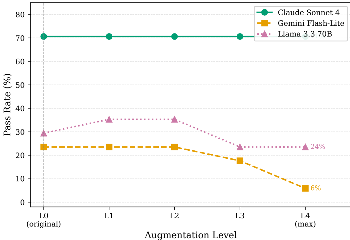
Augmentation Robustness: Pass Rate across L0-L4 (Rodinia CUDA→OpenMP, 17 kernels, seed=42)
