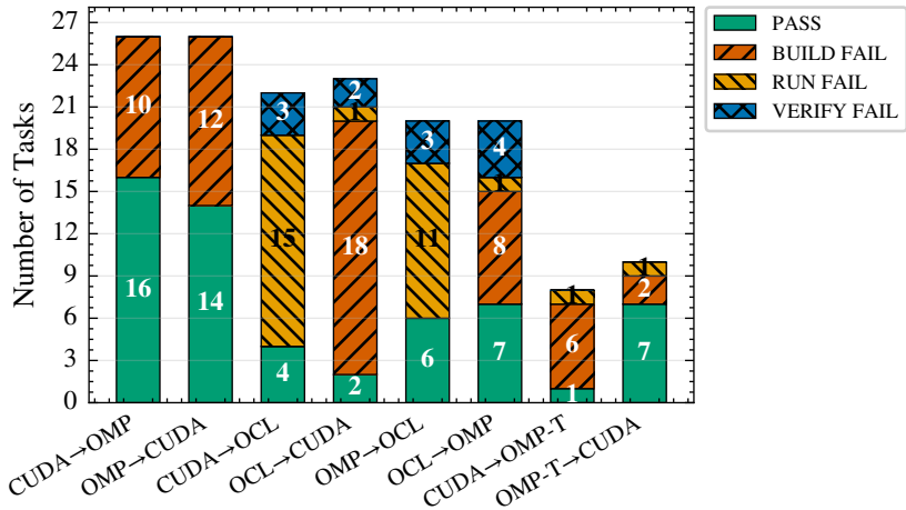
Failure Taxonomy: Status Distribution by Direction (L0, All Suites, Qwen 3.5 397B-A17B)
