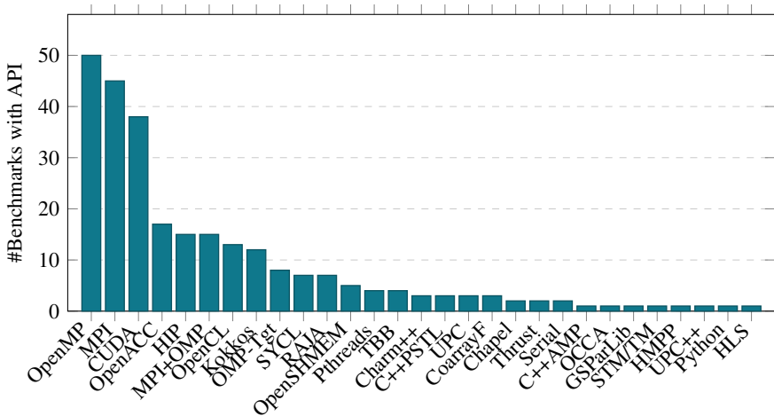
API Coverage Across Surveyed Repositories
