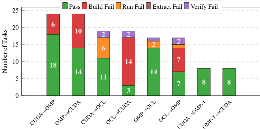
Failure Taxonomy by Direction (GPT-5.3-Codex)
