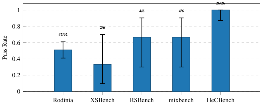
L0 Pass Rate by Suite (GPT-5.3-Codex)
