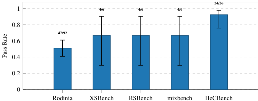
L0 Pass Rate by Suite (GPT-5.4)
