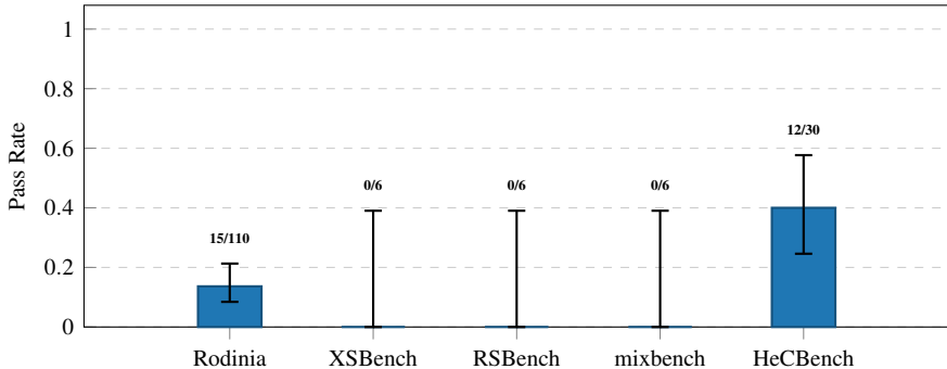
L0 Pass Rate by Suite (Qwen 3.5 397B-A17B)
