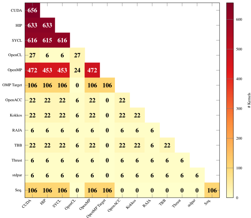
Kernel-Level API Co-occurrence (Number of Kernels with Both APIs)
