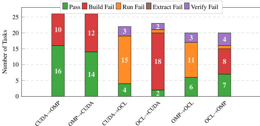
Failure Taxonomy by Direction (Qwen 3.5 397B)
