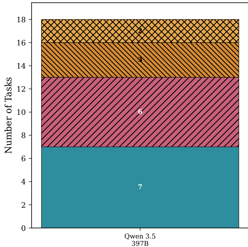
CUDA → OpenMP (L0, 18 kernels)
