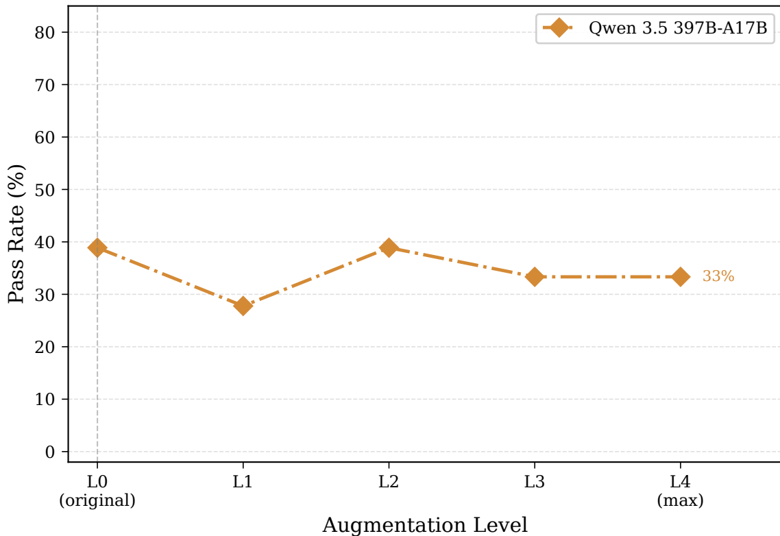
Augmentation Robustness: Pass Rate across L0-L4 (Rodinia CUDA→OpenMP, 18 kernels, seed=42)
