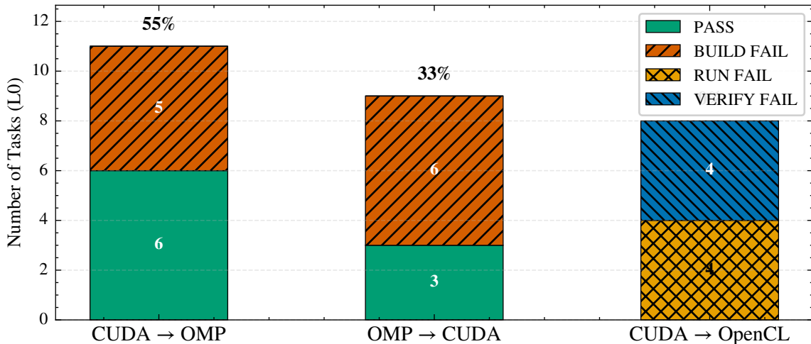
Cross-Direction Status Breakdown (L0, Rodinia) C→O: 11 kernels | O→C: 9 kernels | C→OCL: 8 kernels
