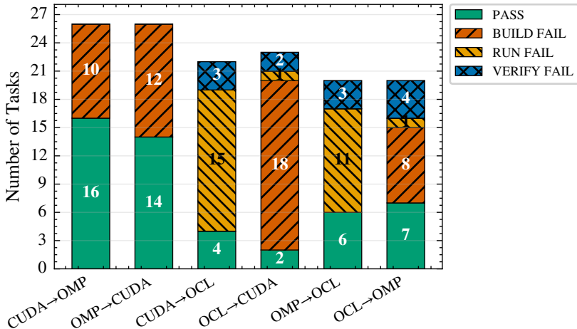
Failure Taxonomy: Status Distribution by Direction (L0, All Suites, Qwen 3.5 397B)
