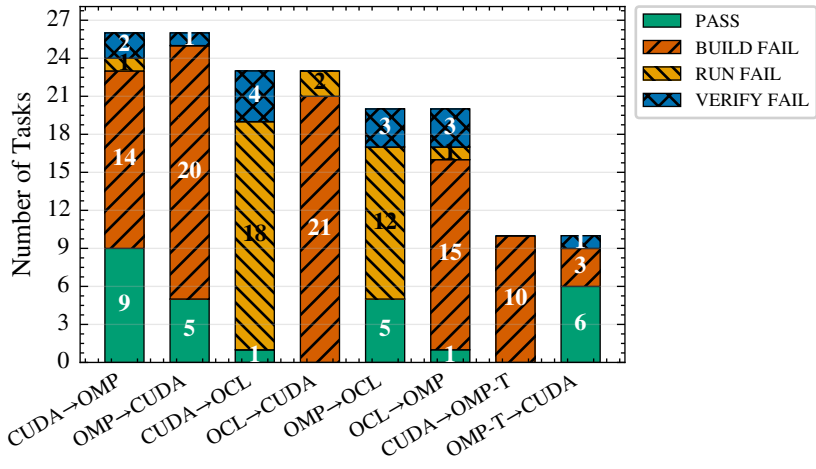
Failure Taxonomy: Status Distribution by Direction (L0, All Suites, Qwen 3.5 397B-A17B)
