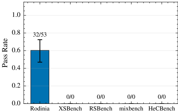
L0 Pass Rate by Suite (Azure GPT-5.4)
