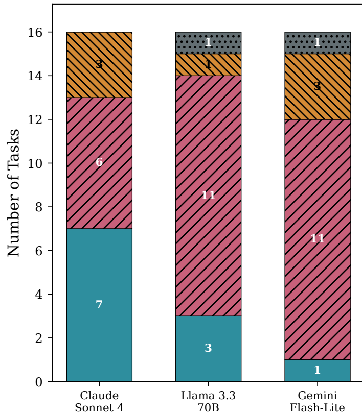
OpenMP → CUDA (L0, 16 kernels)
