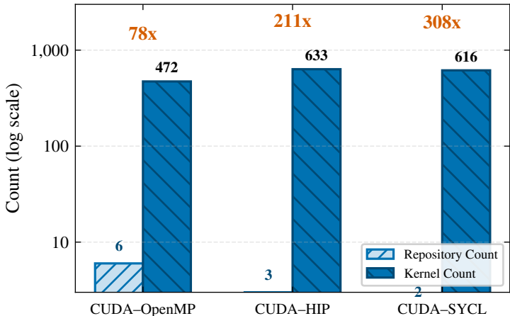
Repo vs. Kernel Translation Pair Counts
