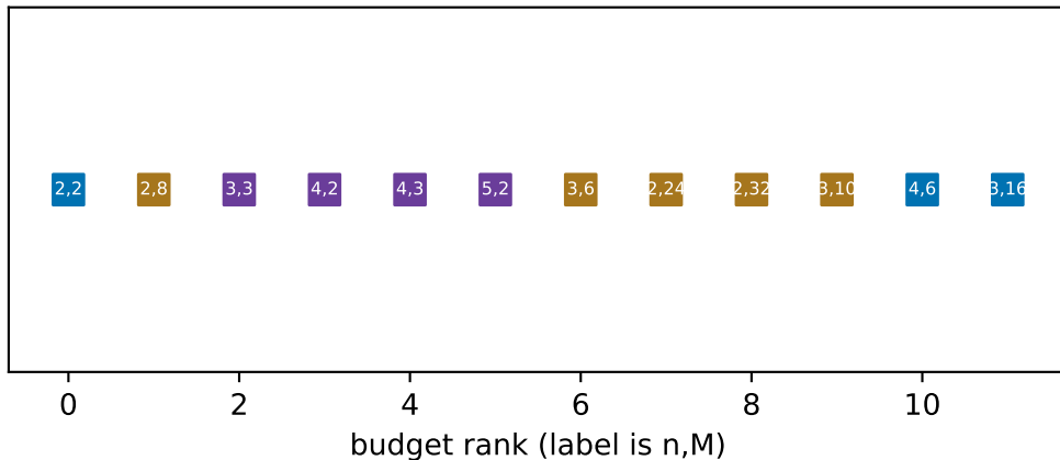
d=80: winning method by increasing stochastic work
