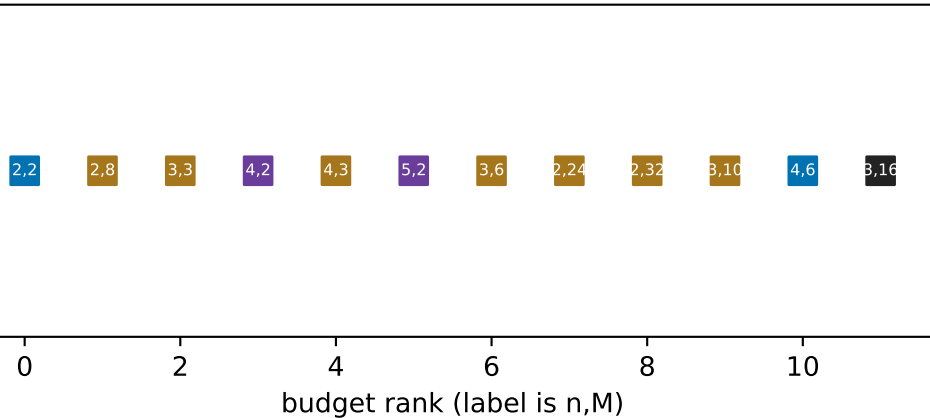
d=60: winning method by increasing stochastic work
