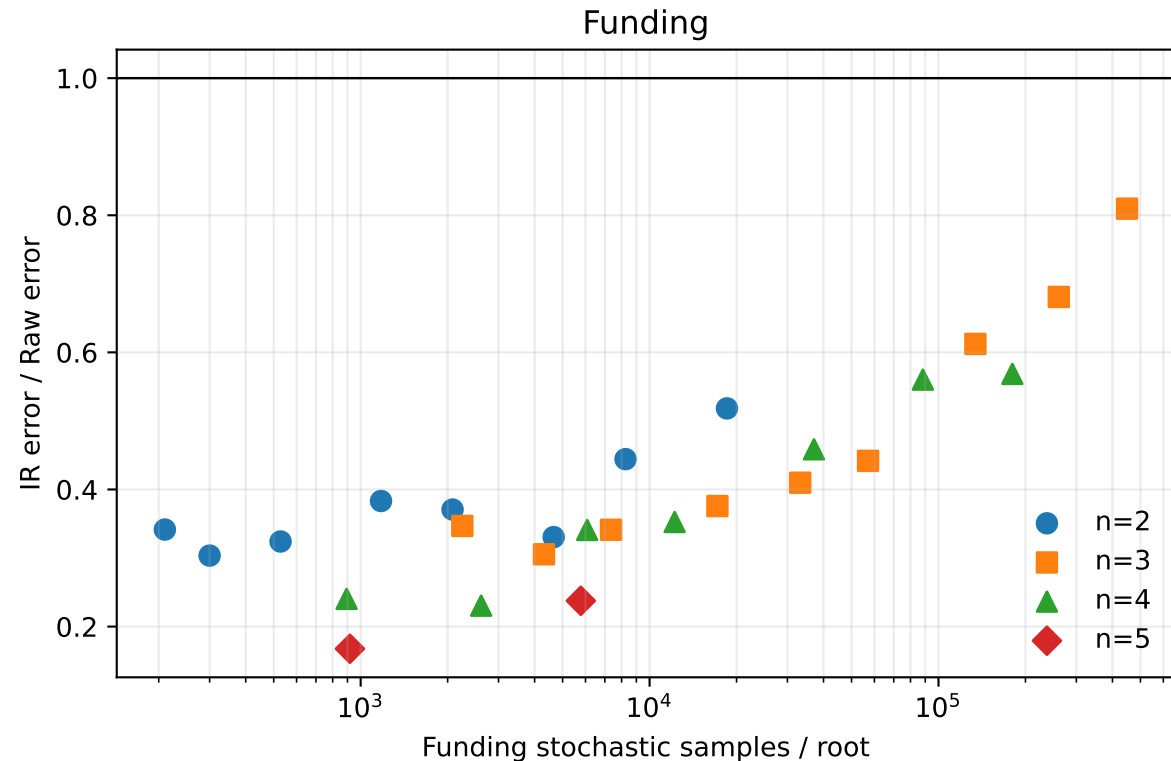
Primary comparison: Samplewise certified IR relative to Raw
