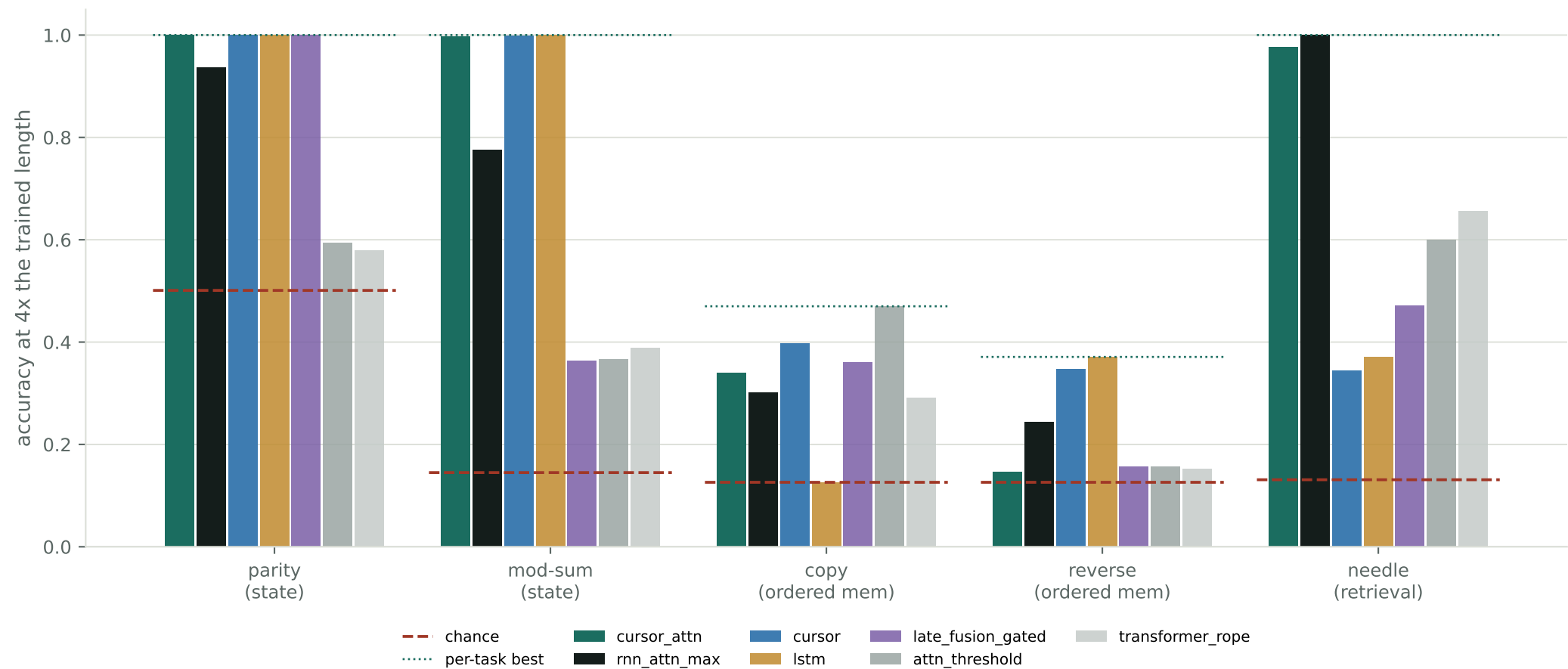
Nova capability frontier — 2400 steps, ~120k parameters, 3 seeds, shortcut-audited tasks
