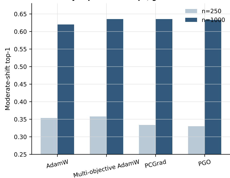
D Auxiliary supervision helps; gradient law does not
