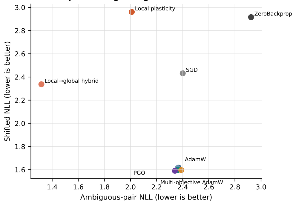
C Local pretraining changes the error tradeoff
