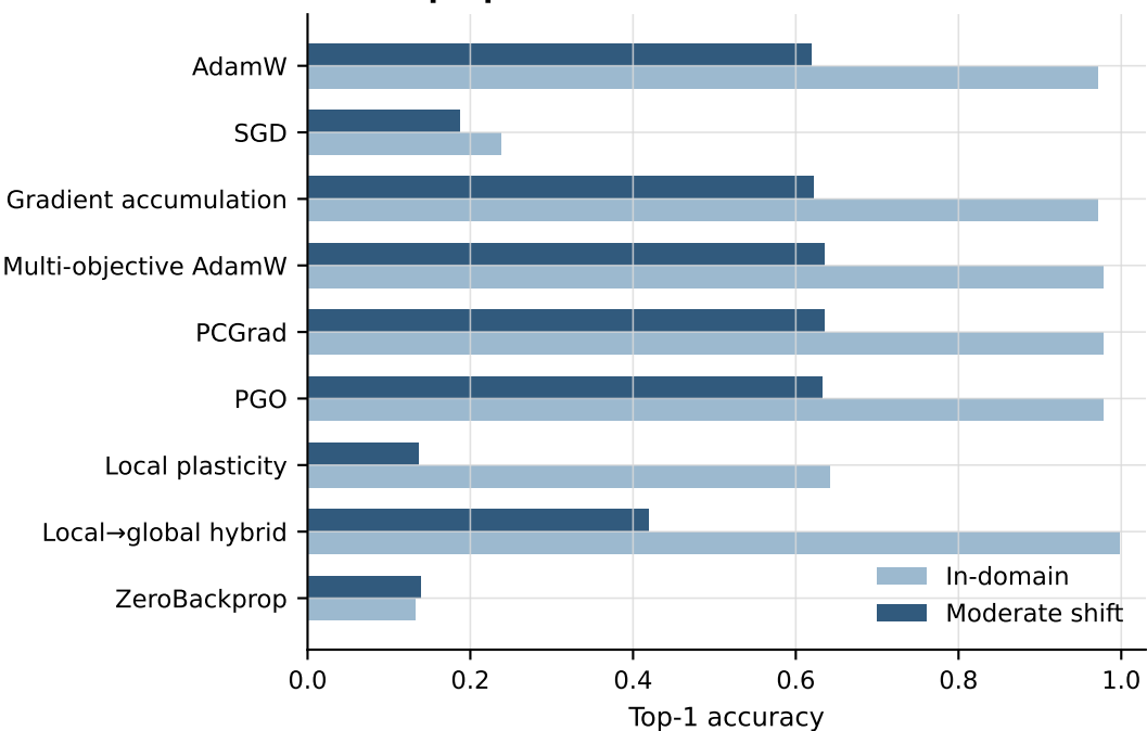
C Local pretraining changes the error tradeoff
