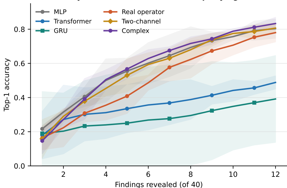
A Accuracy under model-conditioned querying
