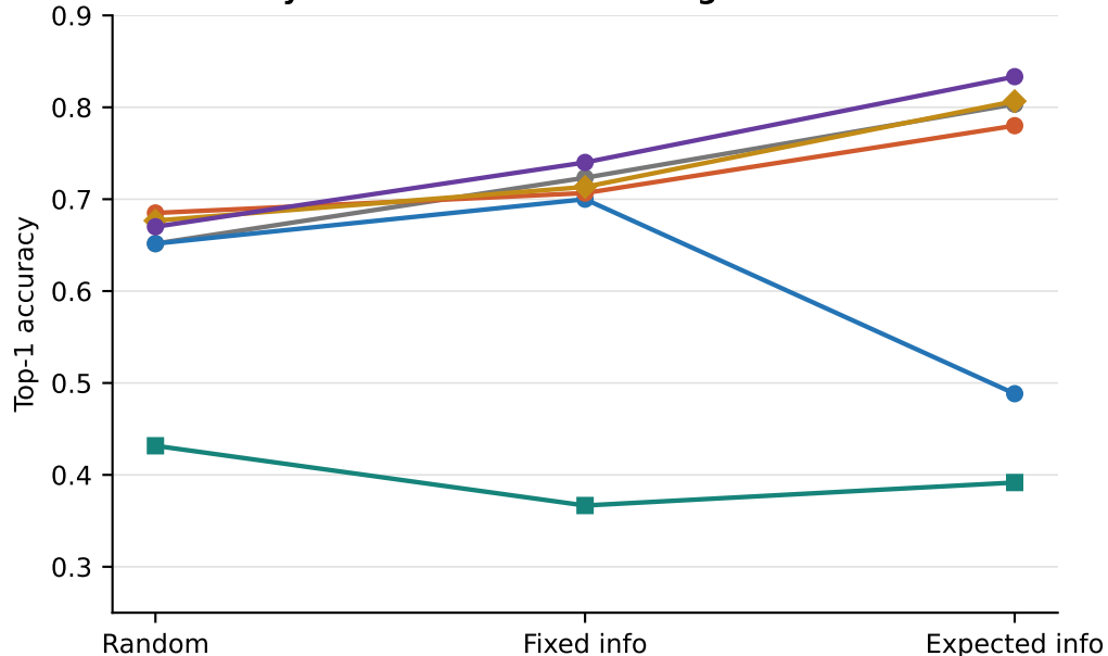
C Accuracy after 12 revealed findings
