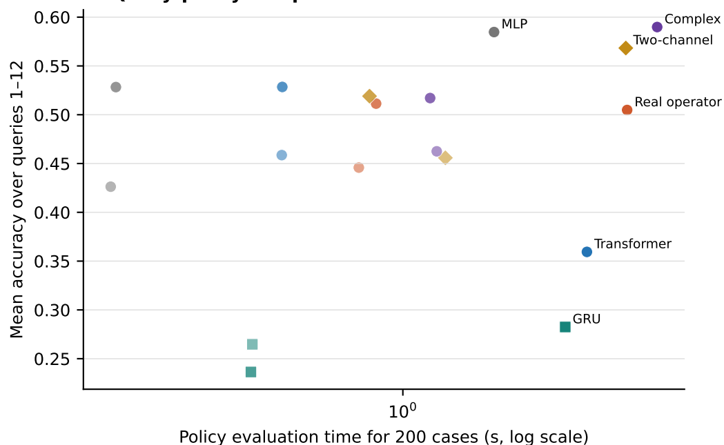
D Query-policy compute frontier
