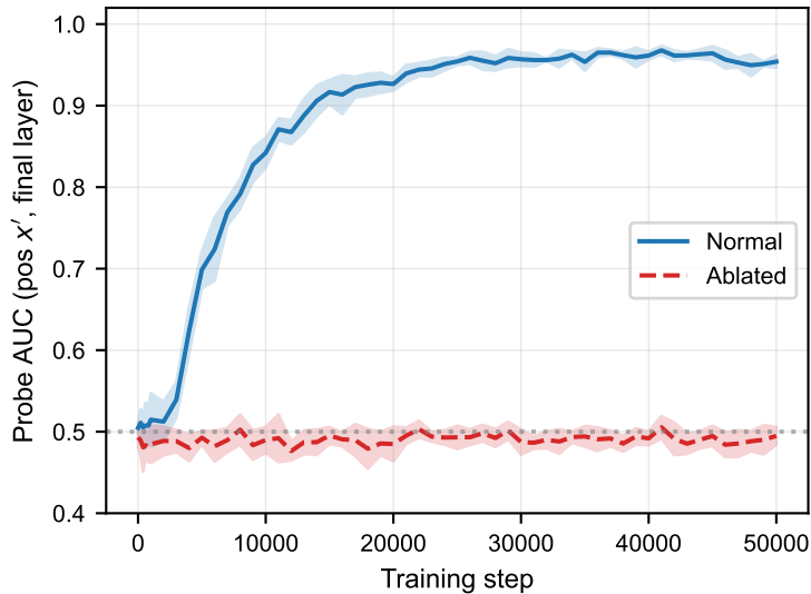
(a) fully-trained, \rho = 0.99 ( n = 5 )
