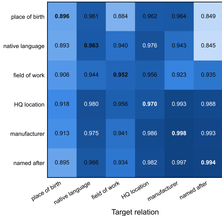
Llama-3.1-8B (layer 7, depth 25%)
