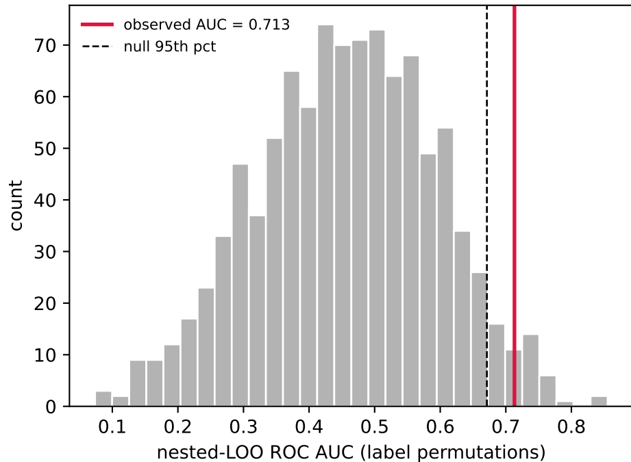
A. Permutation test ( p = 0.027 )
