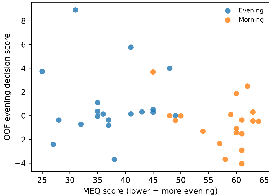
B. Corroboration vs. MEQ ( r = -0.31 , p = 0.057 )
