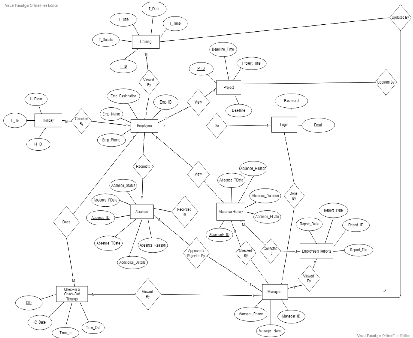
FIGURE 15. ER DIAGRAM FOR BESTFIT APPLICATION
