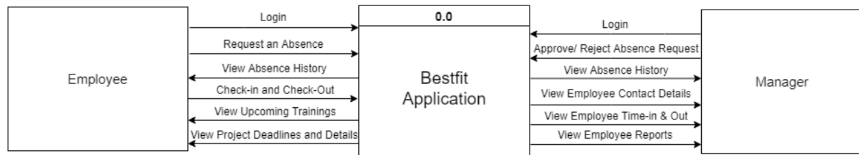
FIGURE 17. DFD DIAGRAM FOR BESTFIT APPLICATION
