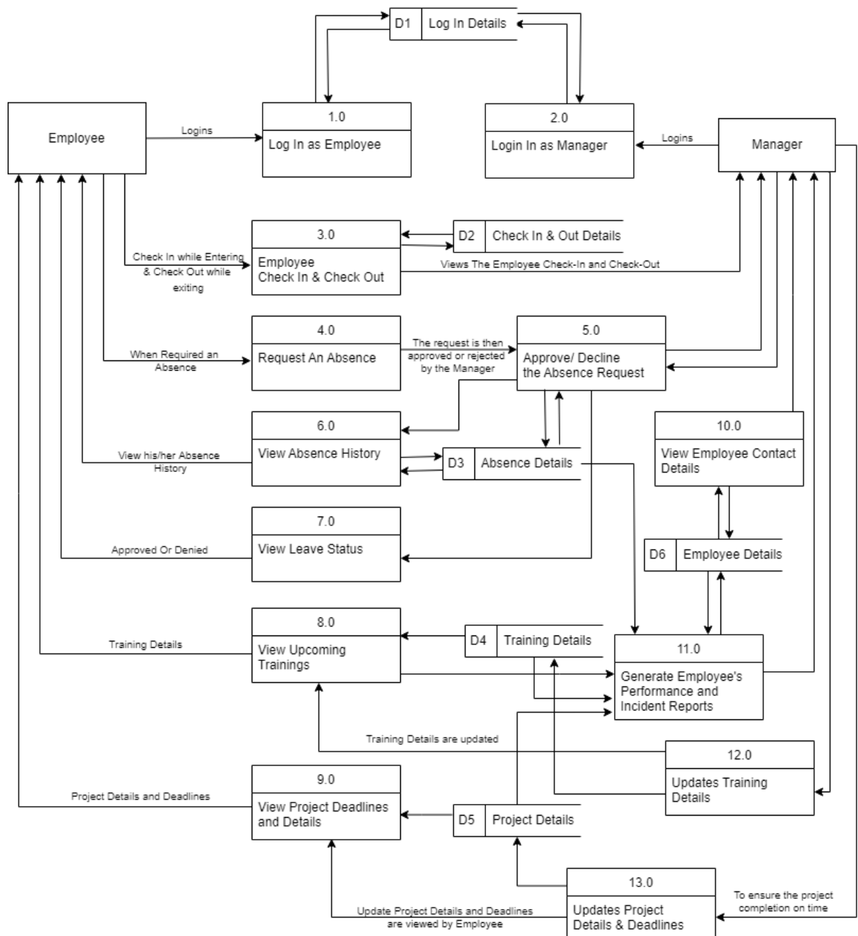
FIGURE 18. DFD DIAGRAM FOR BESTFIT APPLICATION
