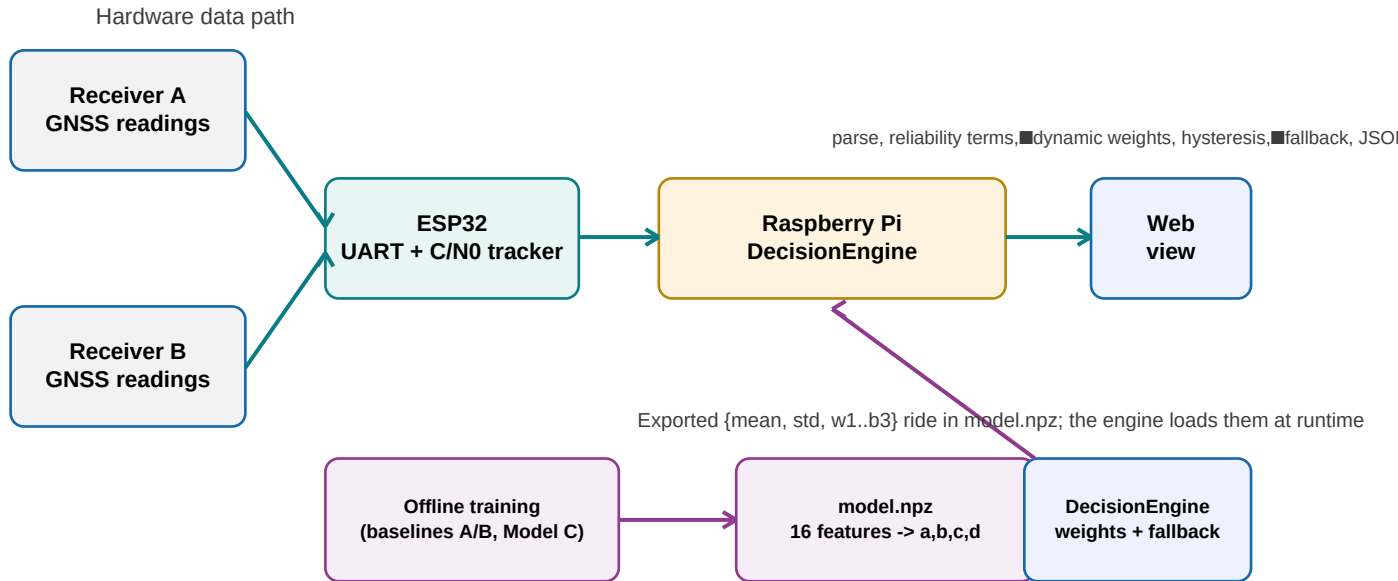
Fig 3.1 The live-integrated pipeline: the exported model drives the Raspberry Pi decision engine.
