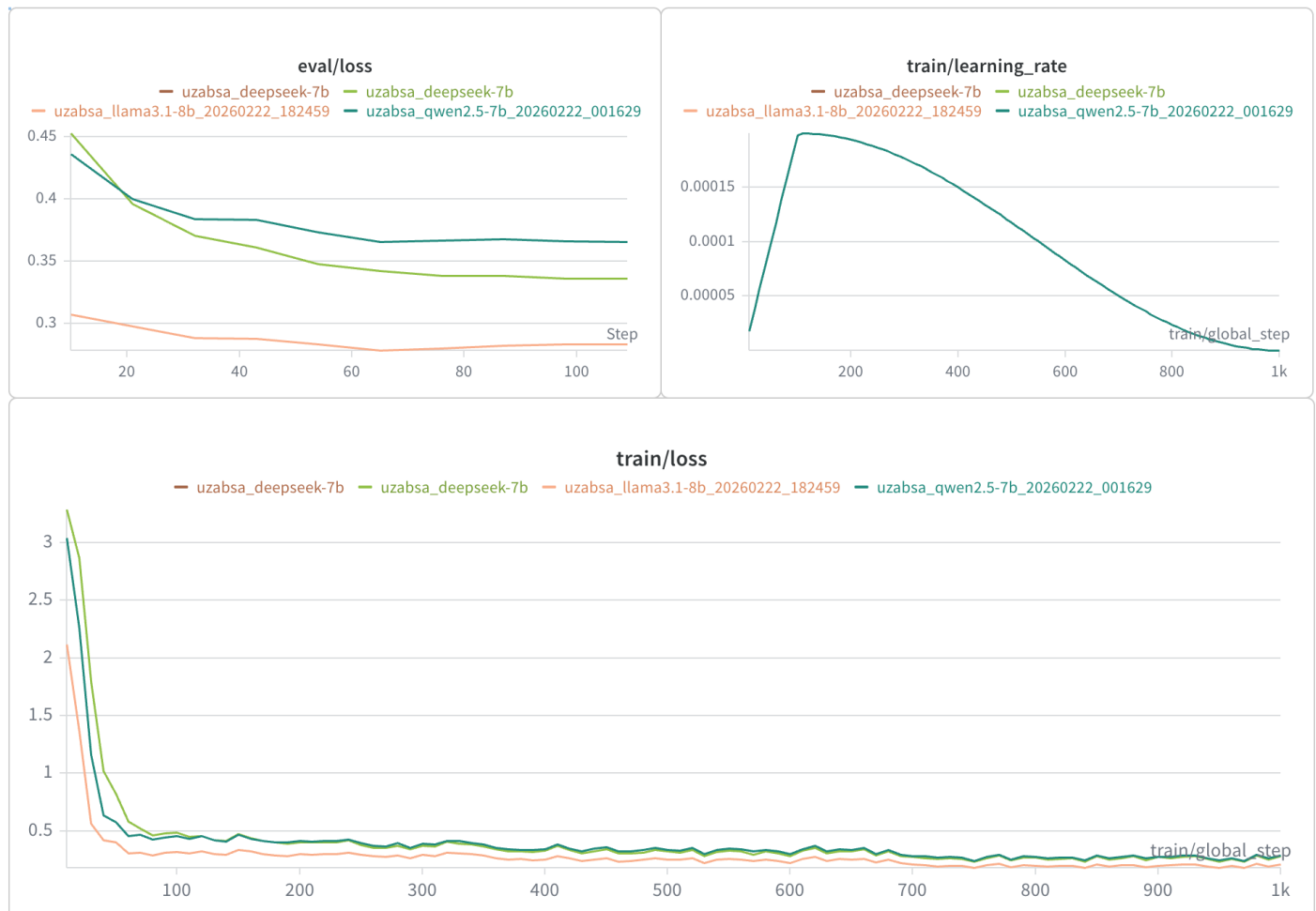
Figure 3. Training dynamics of the three fine-tuned LLMs over 1,000 global steps. (a) Validation loss curves for Qwen 2.5-7B, Llama 3.1-8B, and DeepSeek-R1-Distill-Qwen-7B. (b) Learning-rate schedule used during fine-tuning. (c) Training loss curves for the three models.
