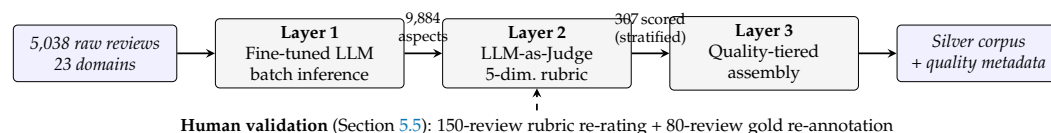
Figure 2. The three-layer model-assisted annotation pipeline. A locally fine-tuned LLM annotates the full multi-domain corpus; an external LLM judge scores a stratified sample on a five-dimension rubric; assembly partitions the corpus into quality tiers. A native-speaker validation study (dashed) calibrates the judge and contributes a reconciled double-annotated subset.
