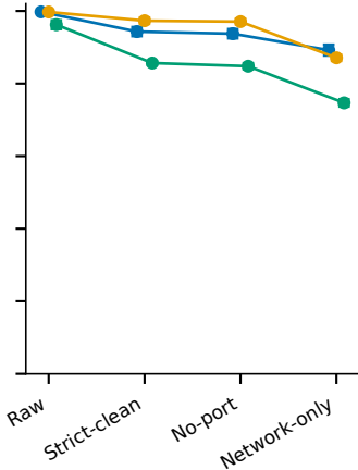
X-IIoTID
