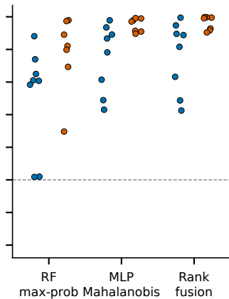
X-IIoTID
