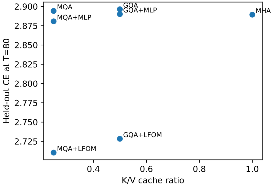
Cache-quality frontier
