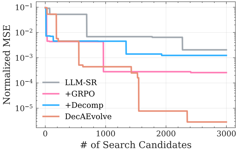
Oscillator1, Qwen2.5-0.5B
