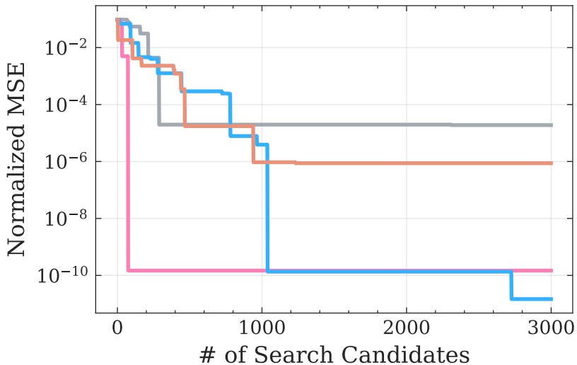
Oscillator1, Qwen2.5-1.5B
