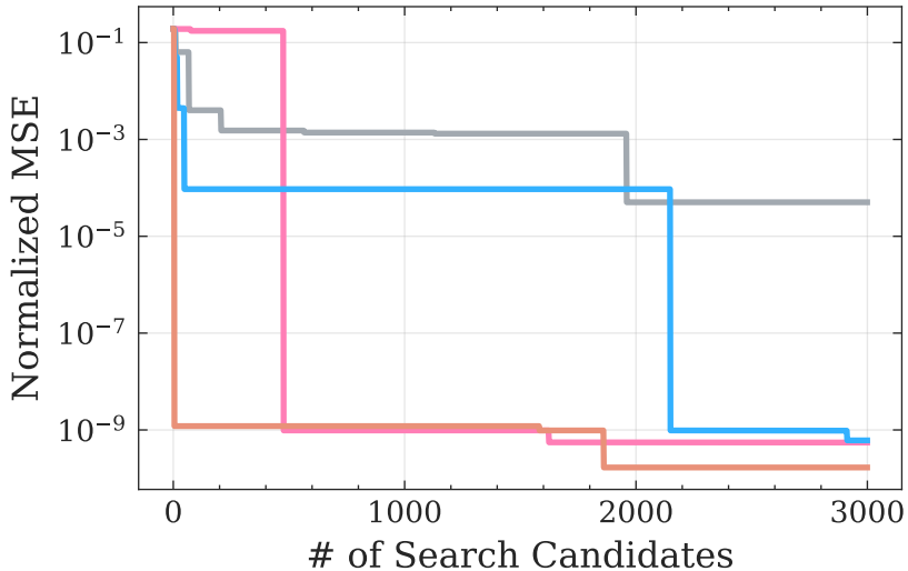
Oscillator2, Qwen2.5-1.5B
