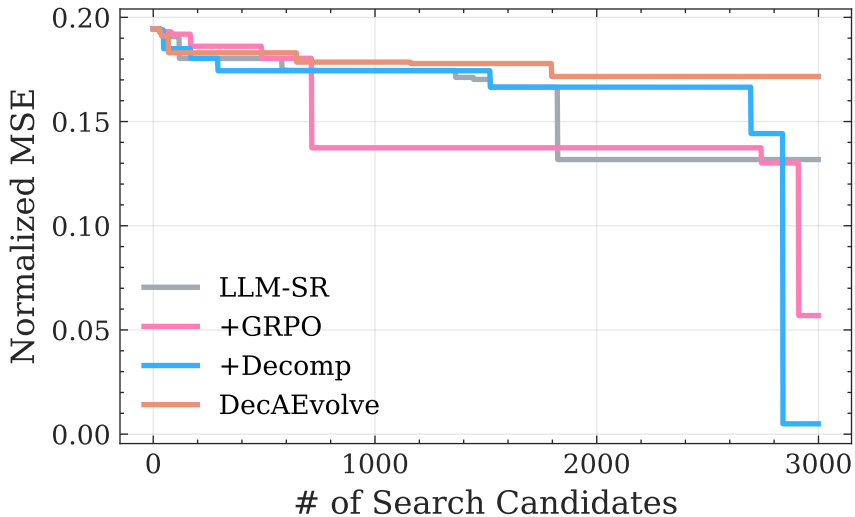
Oscillator2, Qwen2.5-0.5B
