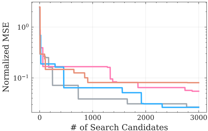
StressStrain, Qwen2.5-1.5B
